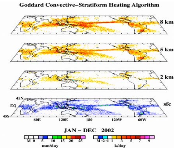
Fig. 4. Latent heating as a function of altitude for 2002 based on CSH algorithm.
