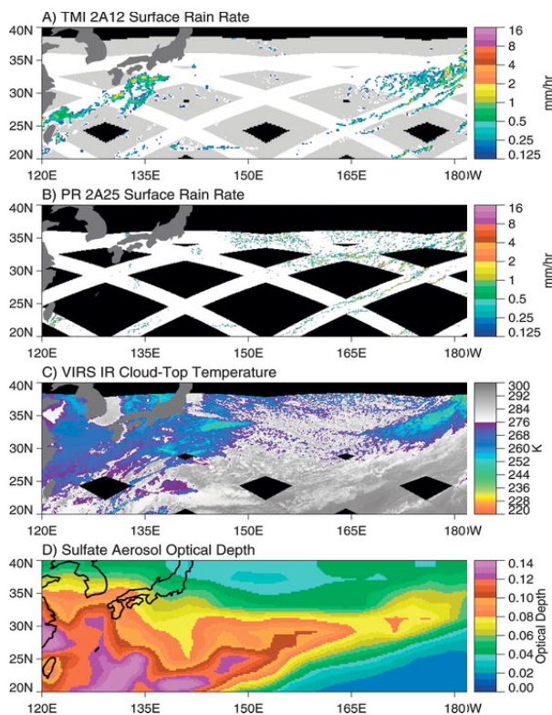
Fig. 9. (a) TMI 2A12 rainfall, (b) PR 2A25 rainfall, (c) VIRS cloud-top temperatures, and (d) model-derived sulfate aerosol optical depth for 1 Feb 2000. The nonraining portions of the TMI scan outside of the PR scan in (a) are gray; nonraining TMI pixels within the PR scan are white. (From Berg et al. 2006)
