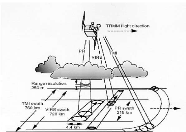
Fig. 1. Schematic of TRMM satellite and scanning geometries of three rain package instruments.
