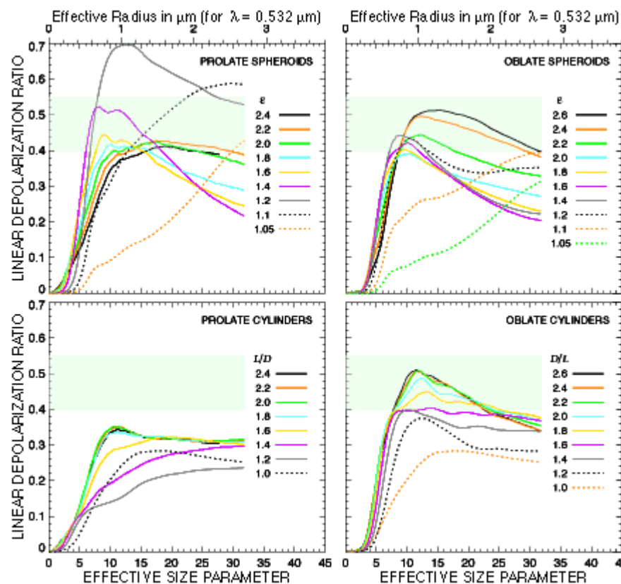
Figure 2. The depolarization ratio as a function of the ice crystal effective size parameter (defined as the average particle circumference divided by the wavelength of light). The upper horizontal axes convert the effective size parameter into the effective radius assuming a lidar wavelength of 0.532 \mu\text{m} . Non-spherical ice crystals are modeled as spheroids with varying axial ratios \epsilon and cylinders with different length-to-diameter ( L/D ) and diameter-to-length ( D/L ) ratios. The light green area shows the highest range of depolarization measured for contrails.
