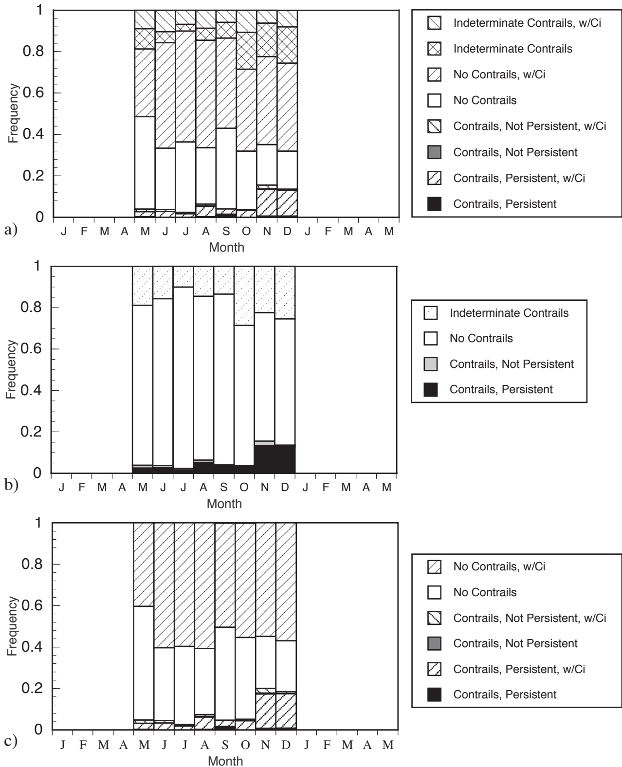
Figure A3. Summary of monthly observations for Cairns AAF, Alabama from January 93 to May 94: (a) relative frequency of contrails and cirrus, (b) relative frequency and persistence of contrails, and (c) relative frequency of contrails and cirrus with indeterminate data removed.
