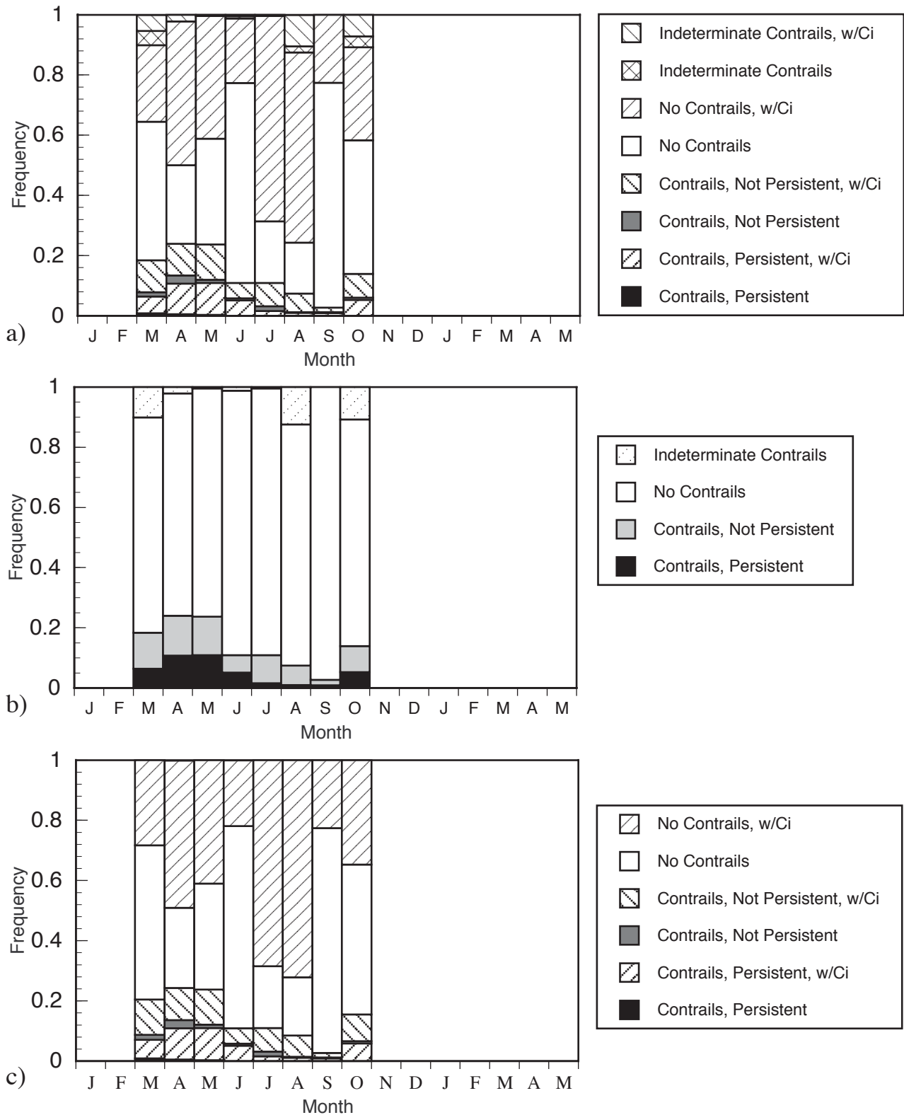
Figure A12. Summary of monthly observations for Luke AFB, Arizona from January 93 to May 94: (a) relative frequency of contrails and cirrus, (b) relative frequency and persistence of contrails, and (c) relative frequency of contrails and cirrus with indeterminate data removed.
