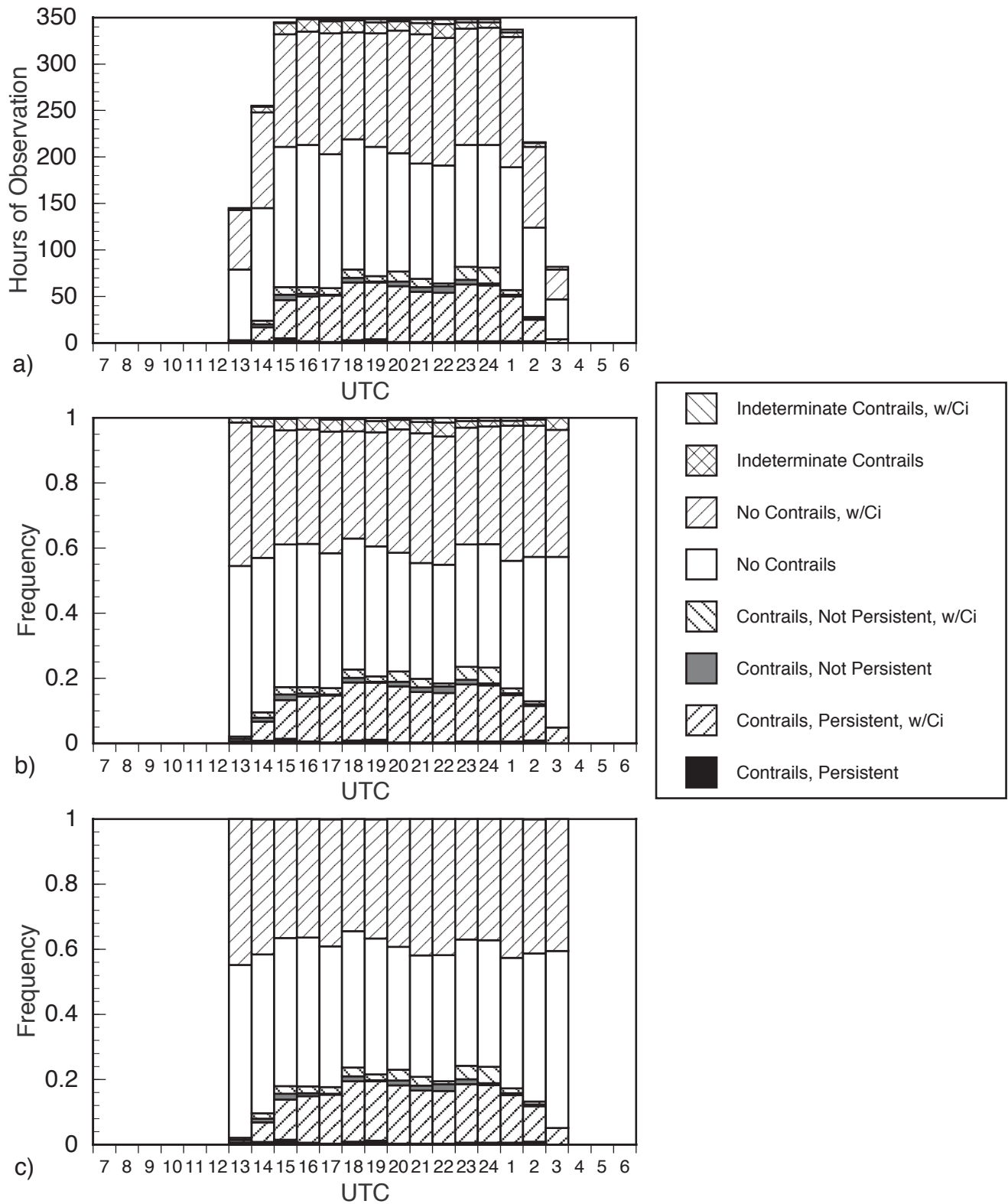
Figure B4. Summary of hourly contrail and cirrus observations from Edwards AFB, California, centered at local noon: (a) number of observations, (b) relative frequency of occurrence, and (c) relative frequency of occurrence with indeterminate data removed.
