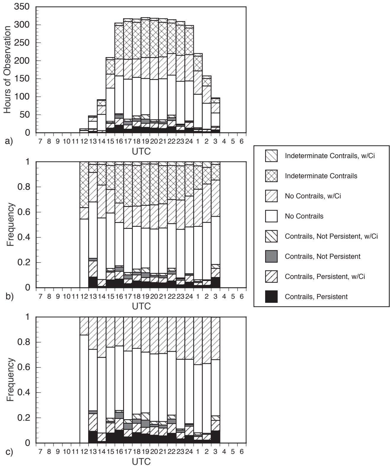
Figure B6. Summary of hourly contrail and cirrus observations from Fairchild AFB, Washington, centered at local noon: (a) number of observations, (b) relative frequency of occurrence, and (c) relative frequency of occurrence with indeterminate data removed.
