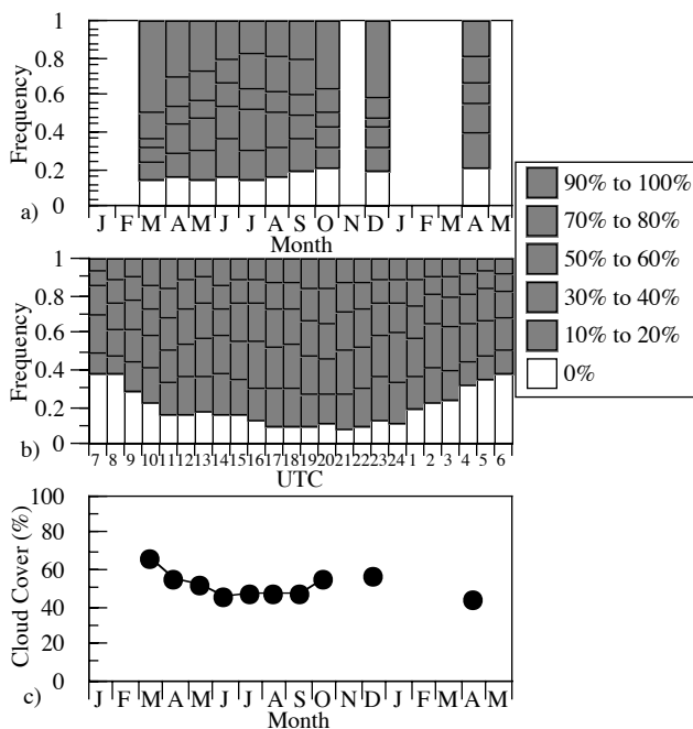
Figure 5. Summary of cloud cover for Langley AFB, Virginia from January 93 to May 94: (a) relative frequency of cloud cover, (b) diurnal cycle of cloud cover relative frequency centered at local noon, and (c) monthly mean cloud cover.
