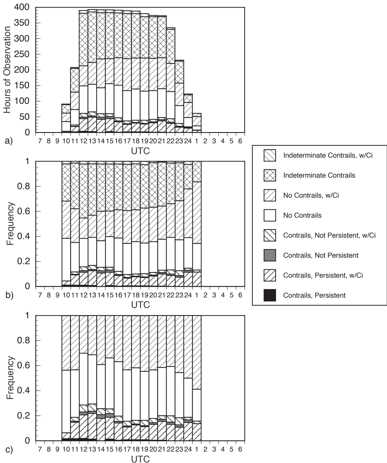
Figure B7. Summary of hourly contrail and cirrus observations from Griffis AFB, New York, centered at local noon: (a) number of observations, (b) relative frequency of occurrence, and (c) relative frequency of occurrence with indeterminate data removed.
