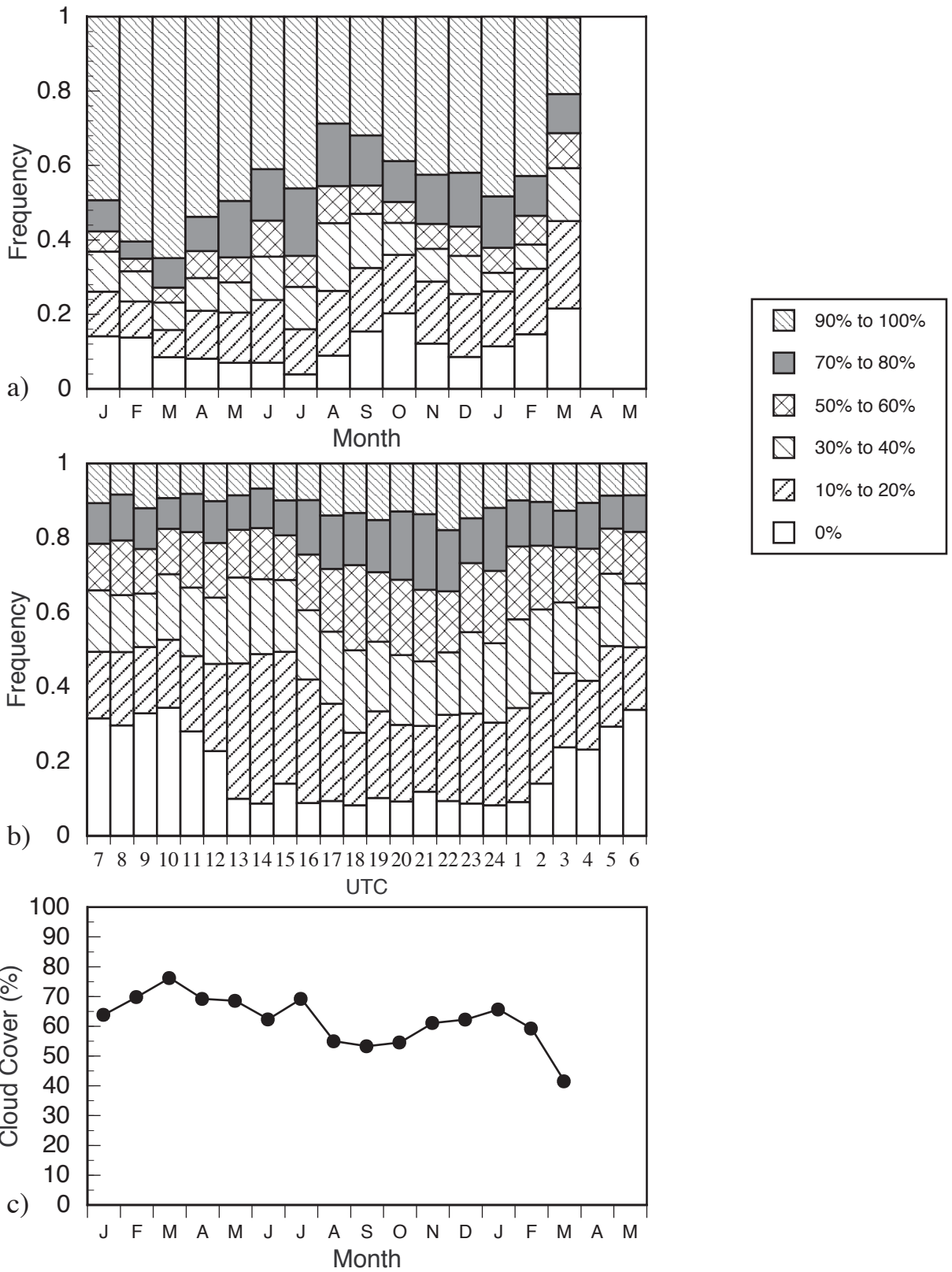
Figure C16. Summary of cloud cover for Offut AFB, Nebraska from January 93 to May 94: (a) relative frequency of cloud cover, (b) diurnal cycle of cloud cover relative frequency centered at local noon, and (c) monthly mean cloud cover.
