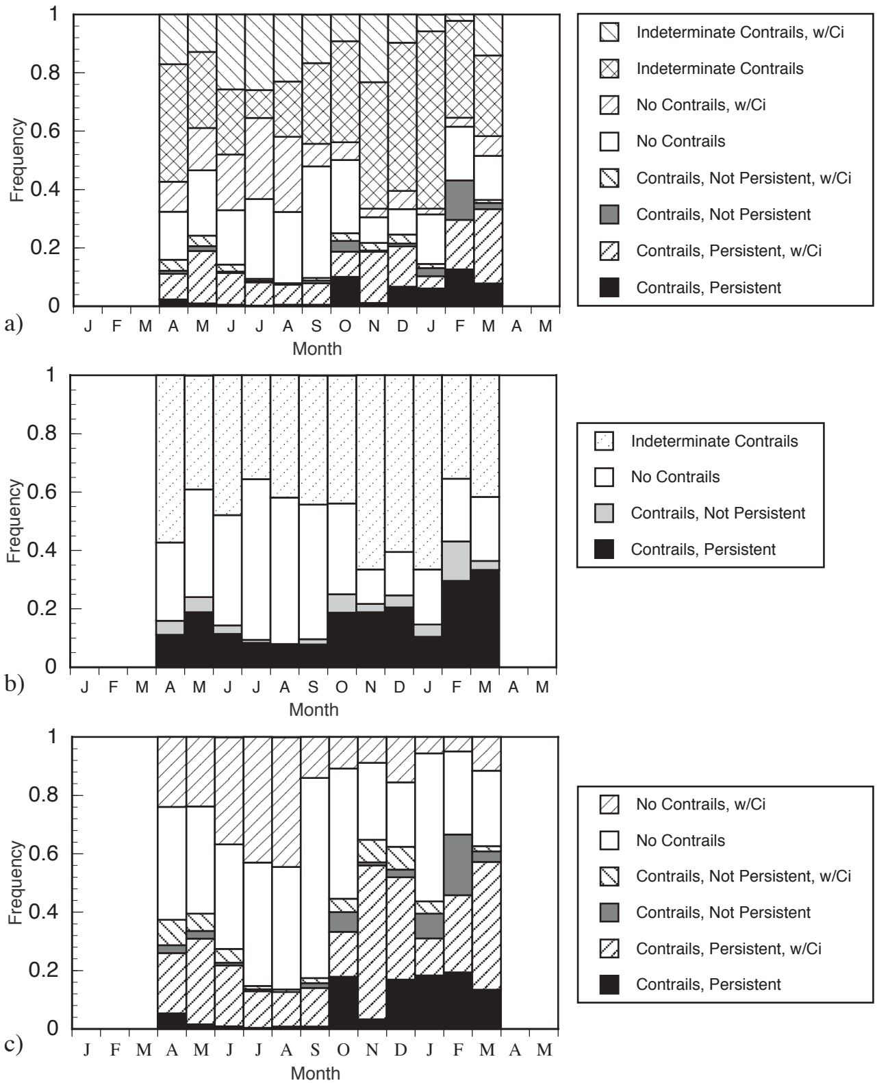
Figure A19. Summary of monthly observations for Wright Patterson AFB, Ohio from January 93 to May 94: (a) relative frequency of contrails and cirrus, (b) relative frequency and persistence of contrails, and (c) relative frequency of contrails and cirrus with indeterminate data removed.
