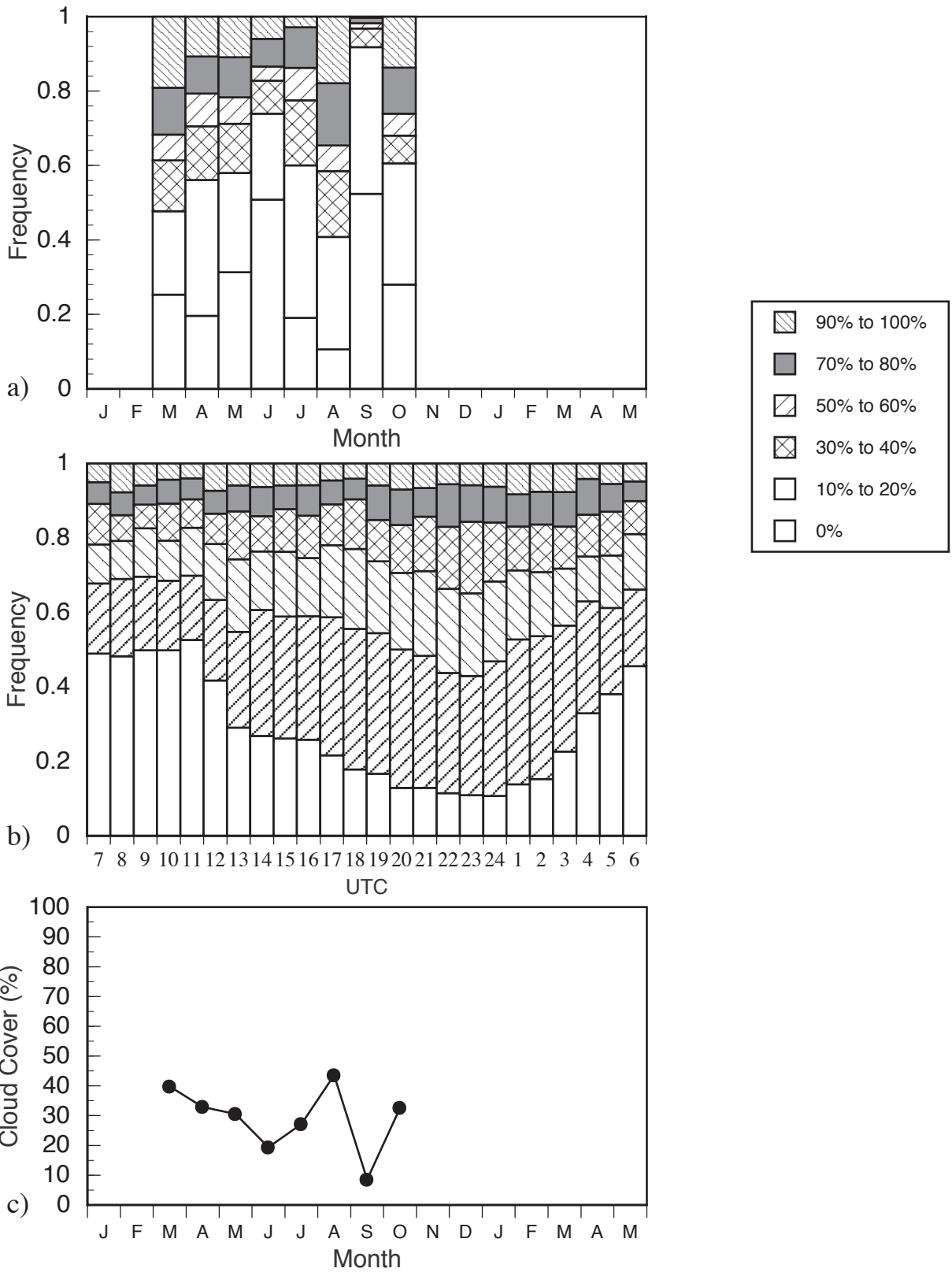
Figure C12. Summary of cloud cover for Luke AFB, Arizona from January 93 to May 94: (a) relative frequency of cloud cover, (b) diurnal cycle of cloud cover relative frequency centered at local noon, and (c) monthly mean cloud cover.
