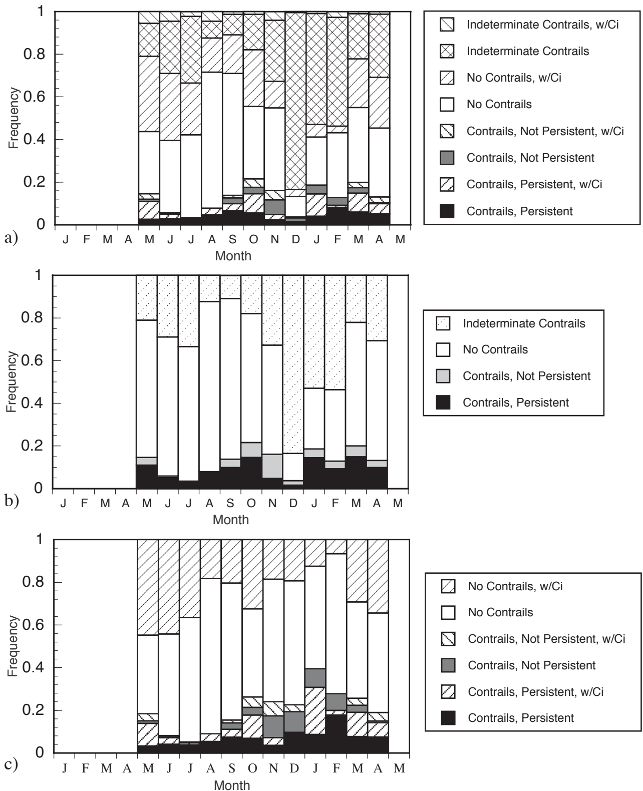
Figure A6. Summary of monthly observations for Fairchild AFB, Washington from January 93 to May 94: (a) relative frequency of contrails and cirrus, (b) relative frequency and persistence of contrails, and (c) relative frequency of contrails and cirrus with indeterminate data removed.
