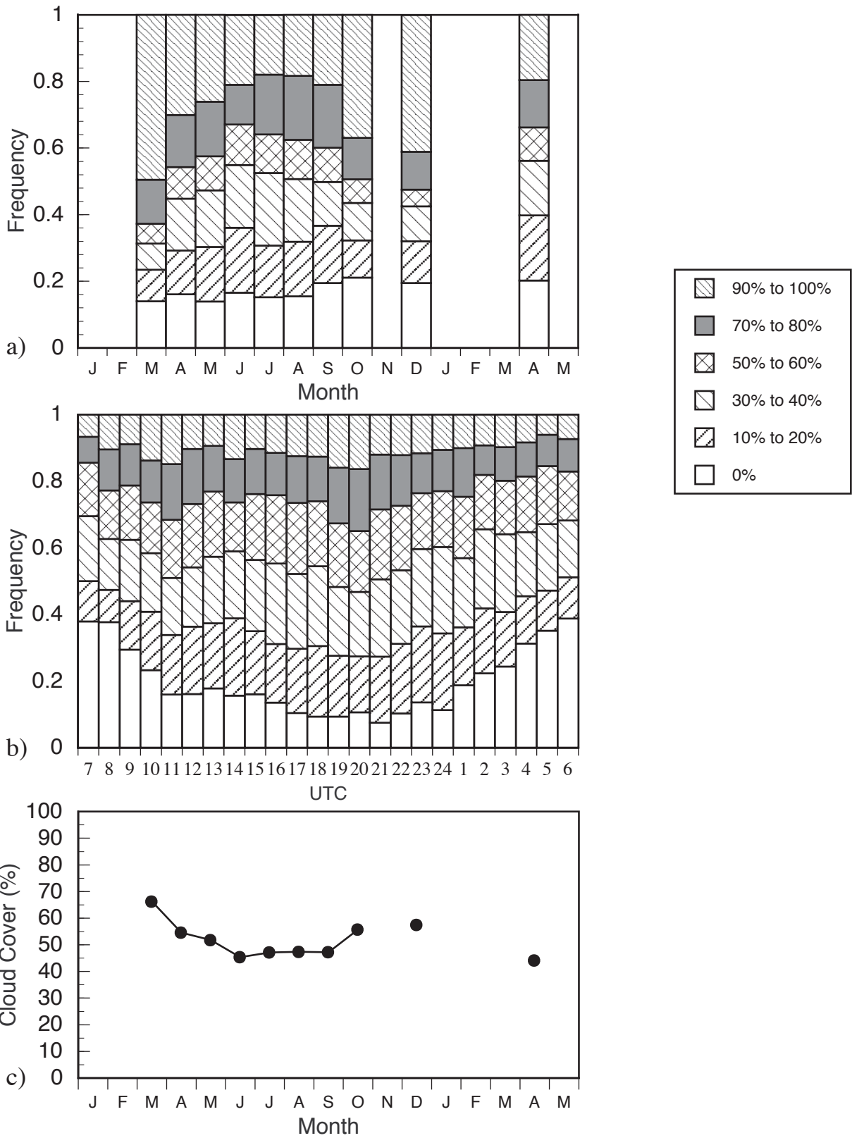
Figure C10. Summary of cloud cover for Langley AFB, Virginia from January 93 to May 94: (a) relative frequency of cloud cover, (b) diurnal cycle of cloud cover relative frequency centered at local noon, and (c) monthly mean cloud cover.
