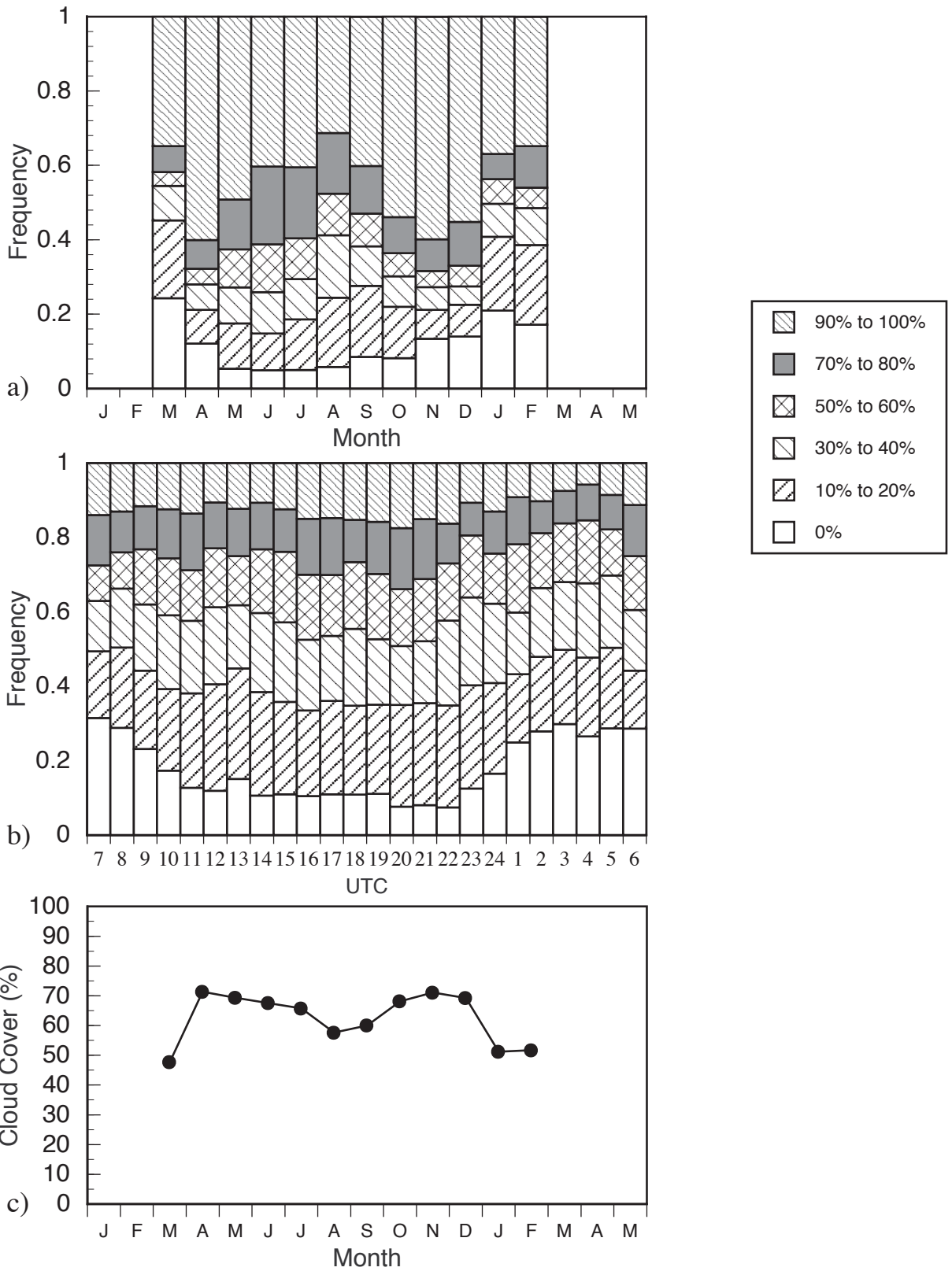
Figure C11. Summary of cloud cover for Loring AFB, Maine from January 93 to May 94: (a) relative frequency of cloud cover, (b) diurnal cycle of cloud cover relative frequency centered at local noon, and (c) monthly mean cloud cover.
