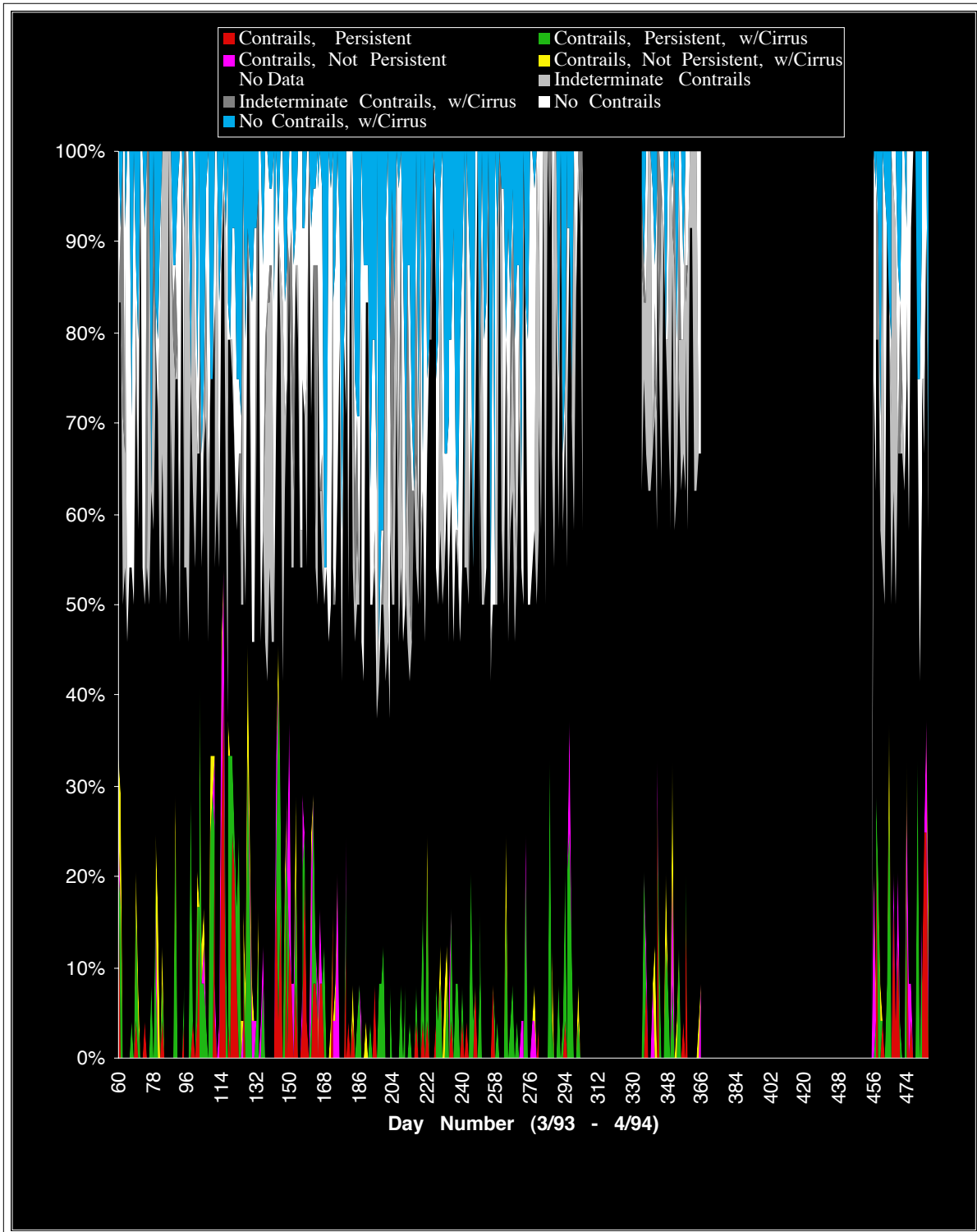
Figure 3. Summary of daily observations over LAFB for the period from March 1993 through April 1994.
