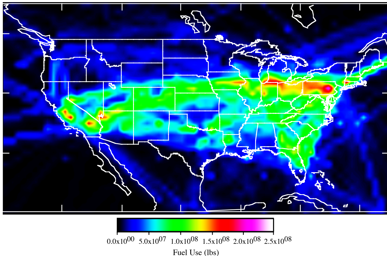
Figure 17. Sum of aircraft fuel usage for altitudes greater than 7 kilometers.
