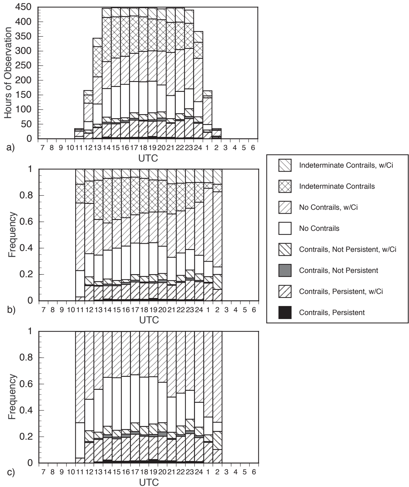
Figure B1. Summary of hourly contrail and cirrus observations from Barksdale AFB, Louisiana, centered at local noon: (a) number of observations, (b) relative frequency of occurrence, and (c) relative frequency of occurrence with indeterminate data removed.
