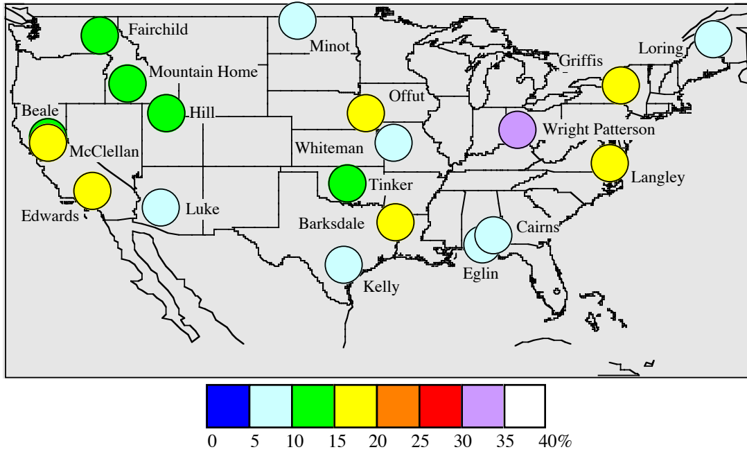
Figure 18. Annual mean persistent contrail frequency excluding indeterminate data for 19 surface observation sites.
