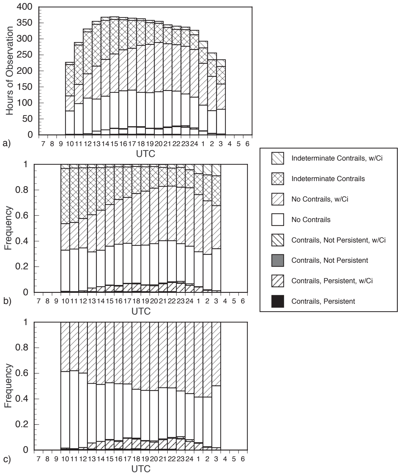
Figure B9. Summary of hourly contrail and cirrus observations from Kelly AFB, Texas, centered at local noon: (a) number of observations, (b) relative frequency of occurrence, and (c) relative frequency of occurrence with indeterminate data removed.
