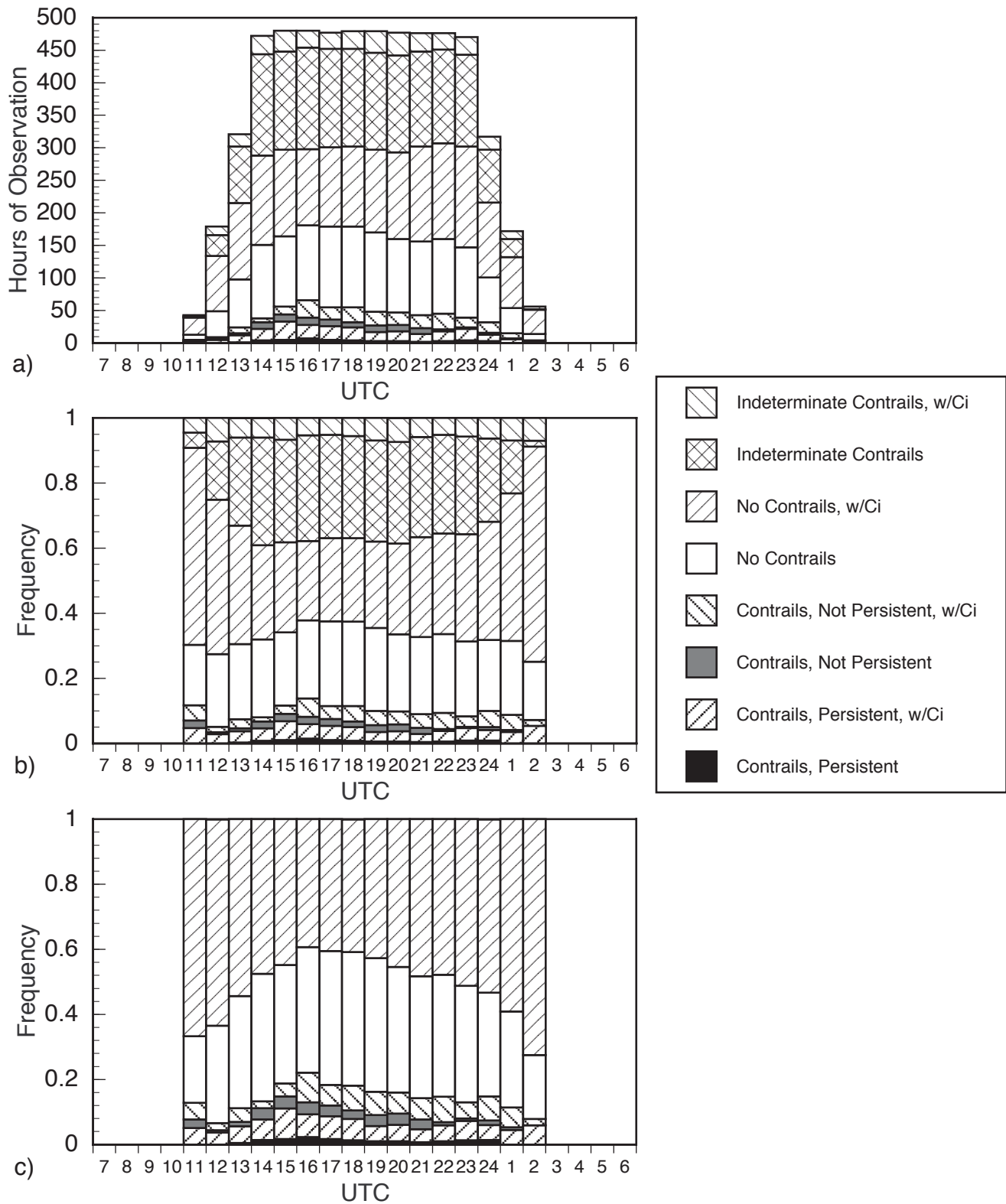
Figure B18. Summary of hourly contrail and cirrus observations from Whiteman AFB, Missouri, centered at local noon: (a) number of observations, (b) relative frequency of occurrence, and (c) relative frequency of occurrence with indeterminate data removed.
