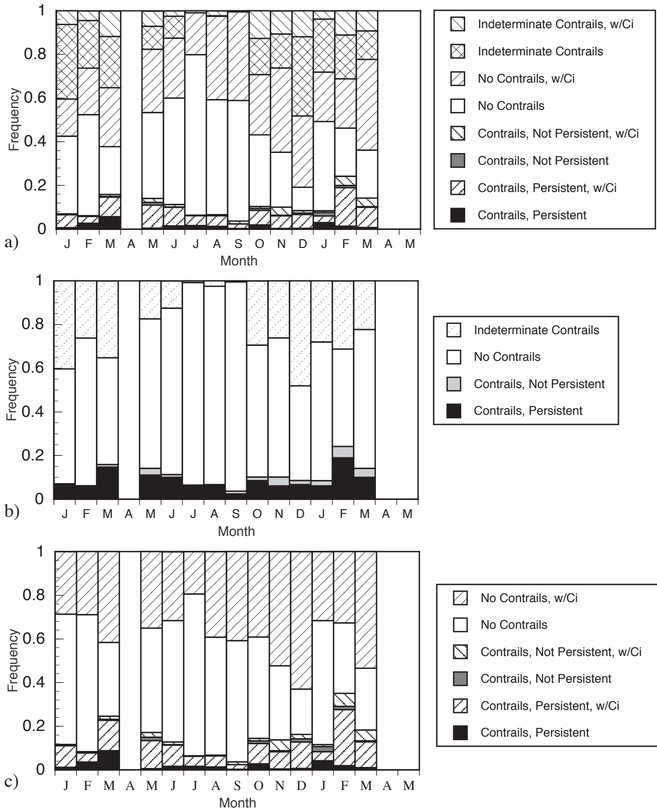
Figure A2. Summary of monthly observations for Beale AFB, California from January 93 to May 94: (a) relative frequency of contrails and cirrus, (b) relative frequency and persistence of contrails, and (c) relative frequency of contrails and cirrus with indeterminate data removed.
