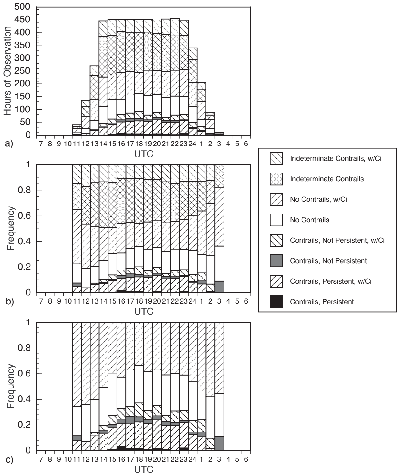
Figure B16. Summary of hourly contrail and cirrus observations from Offut AFB, Nebraska, centered at local noon: (a) number of observations, (b) relative frequency of occurrence, and (c) relative frequency of occurrence with indeterminate data removed.
