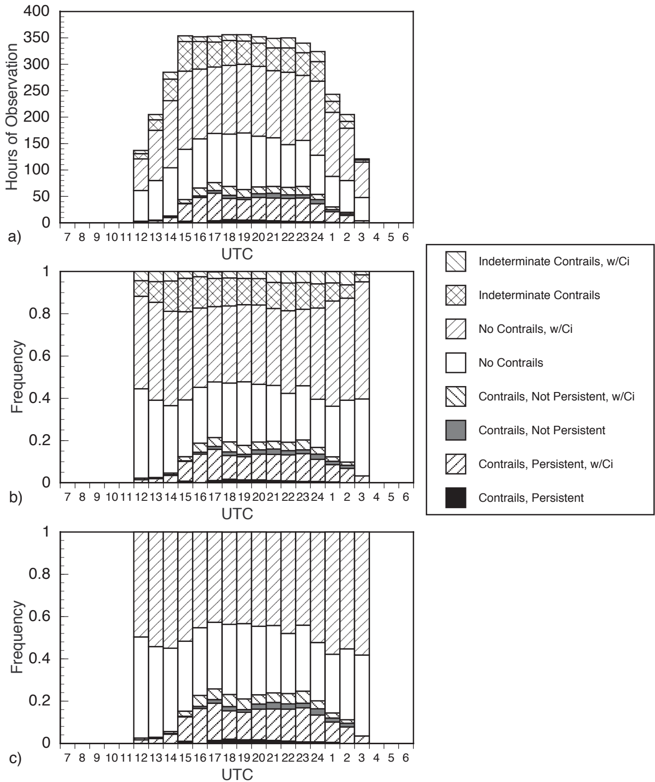
Figure B8. Summary of hourly contrail and cirrus observations from Hill AFB, Utah, centered at local noon: (a) number of observations, (b) relative frequency of occurrence, and (c) relative frequency of occurrence with indeterminate data removed.
