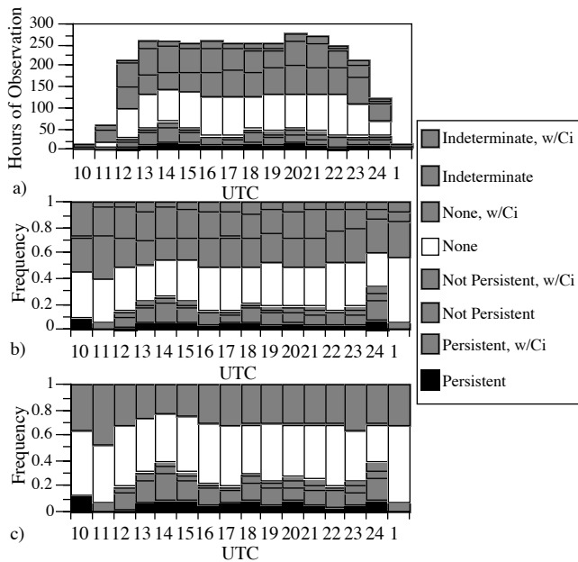
Figure 9. Summary of hourly contrail and cirrus observations from Langley AFB, Virginia, centered at local noon: (a) number of observations, (b) relative frequency of occurrence, and (c) relative frequency of occurrence with indeterminate data removed.
