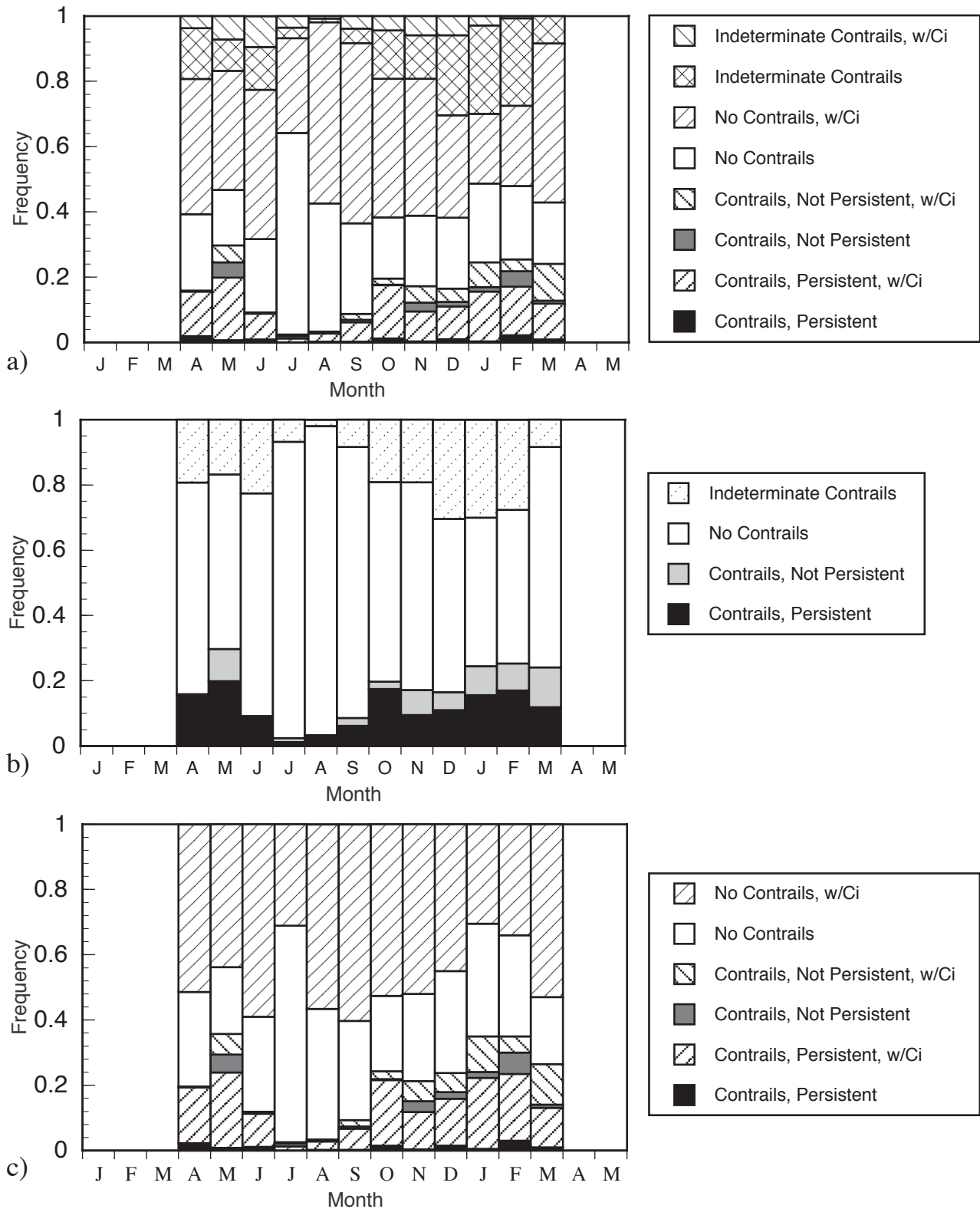
Figure A8. Summary of monthly observations for Hill AFB, Utah from January 93 to May 94: (a) relative frequency of contrails and cirrus, (b) relative frequency and persistence of contrails, and (c) relative frequency of contrails and cirrus with indeterminate data removed.
