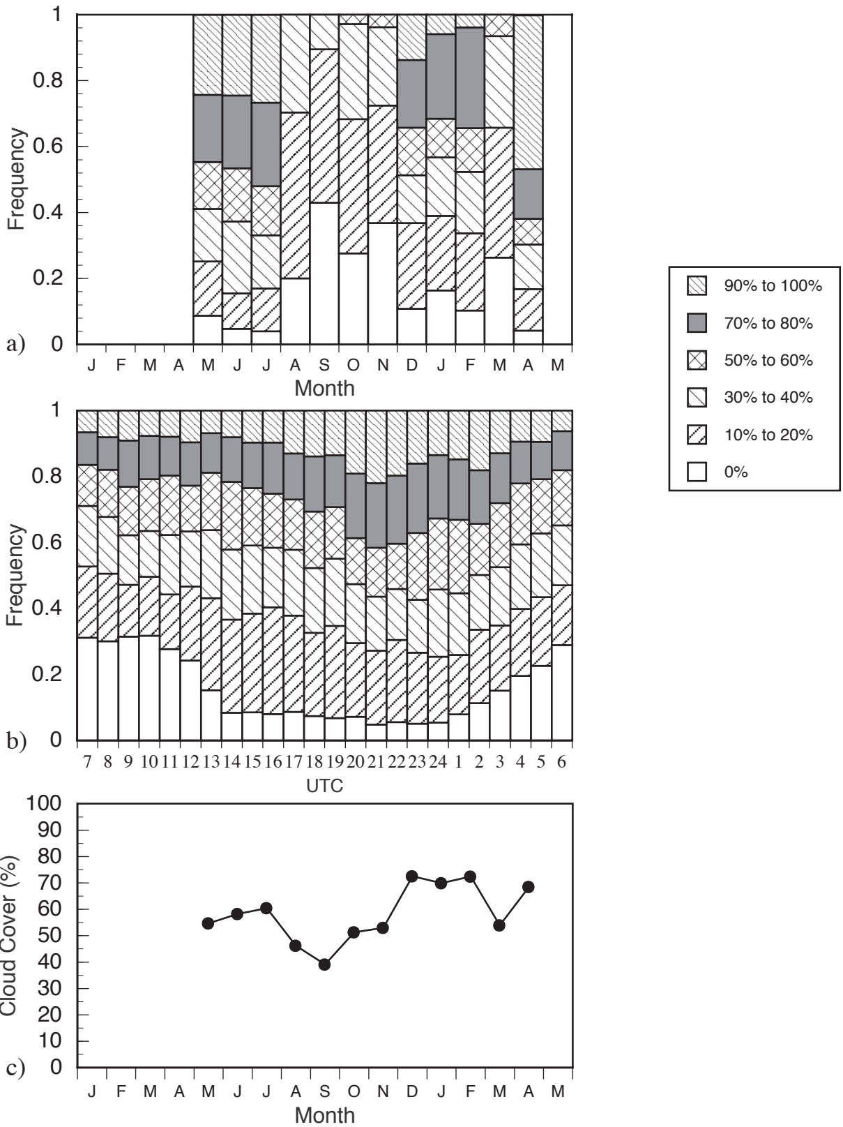
Figure C6. Summary of cloud cover for Fairchild AFB, Washington from January 93 to May 94: (a) relative frequency of cloud cover, (b) diurnal cycle of cloud cover relative frequency centered at local noon, and (c) monthly mean cloud cover.
