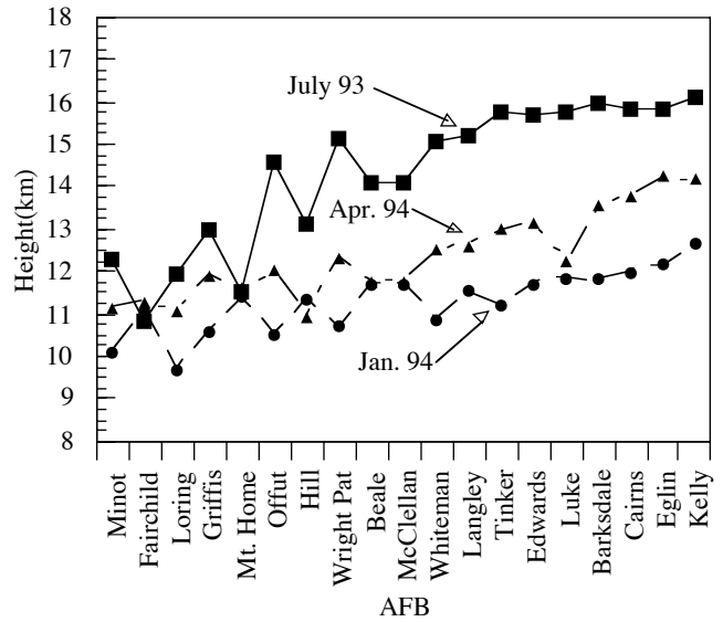
Figure 20. Variation of mean tropopause altitude for July 1993, January 1994, and April 1994. Sites ordered North to South according to latitude.
