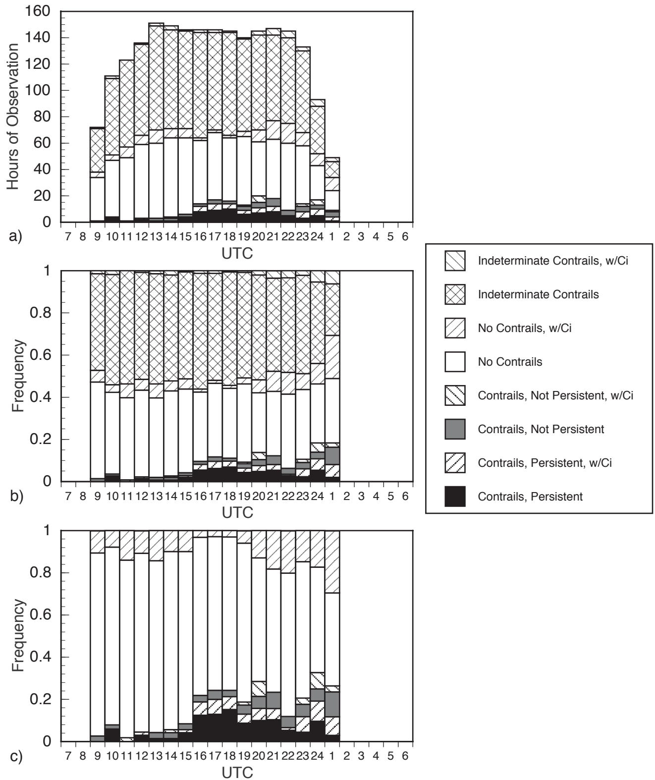
Figure B11. Summary of hourly contrail and cirrus observations from Loring AFB, Maine, centered at local noon: (a) number of observations, (b) relative frequency of occurrence, and (c) relative frequency of occurrence with indeterminate data removed.
