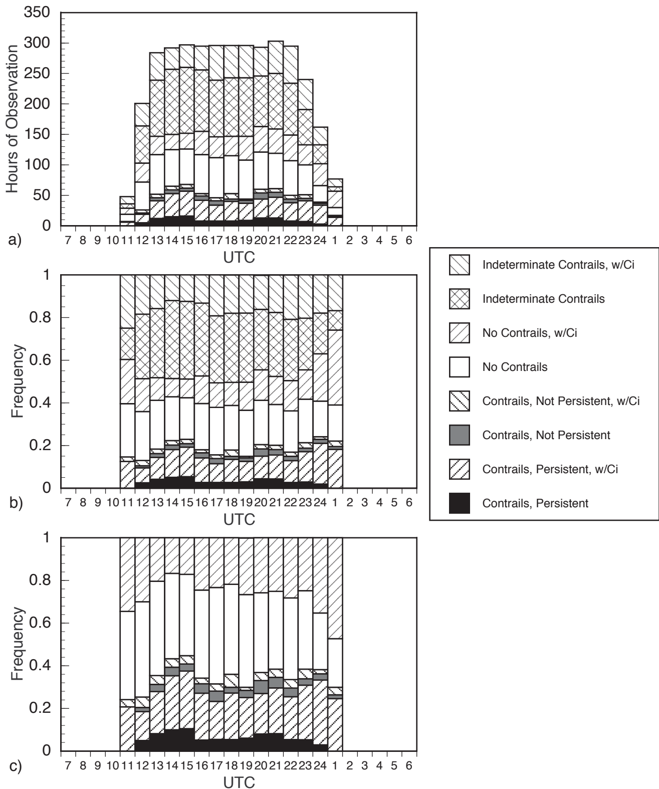
Figure B19. Summary of hourly contrail and cirrus observations from Wright Patterson AFB, Ohio, centered at local noon: (a) number of observations, (b) relative frequency of occurrence, and (c) relative frequency of occurrence with indeterminate data removed.
