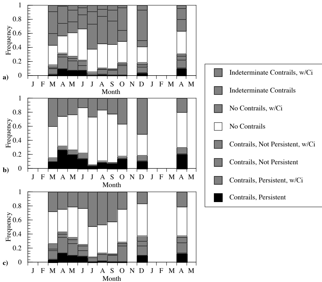
Figure 4. Summary of monthly observations for Langley AFB, Virginia from January 1993 to May 1994: (a) relative frequency of contrails and cirrus, (b) relative frequency and persistence of contrails, and (c) relative frequency of contrails and cirrus with indeterminate data removed.
