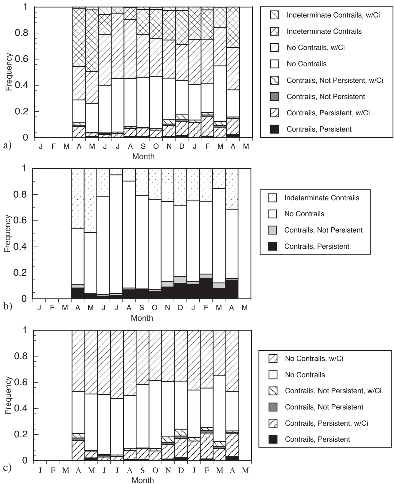
Figure A17. Summary of monthly observations for Tinker AFB, Oklahoma from January 93 to May 94: (a) relative frequency of contrails and cirrus, (b) relative frequency and persistence of contrails, and (c) relative frequency of contrails and cirrus with indeterminate data removed.
