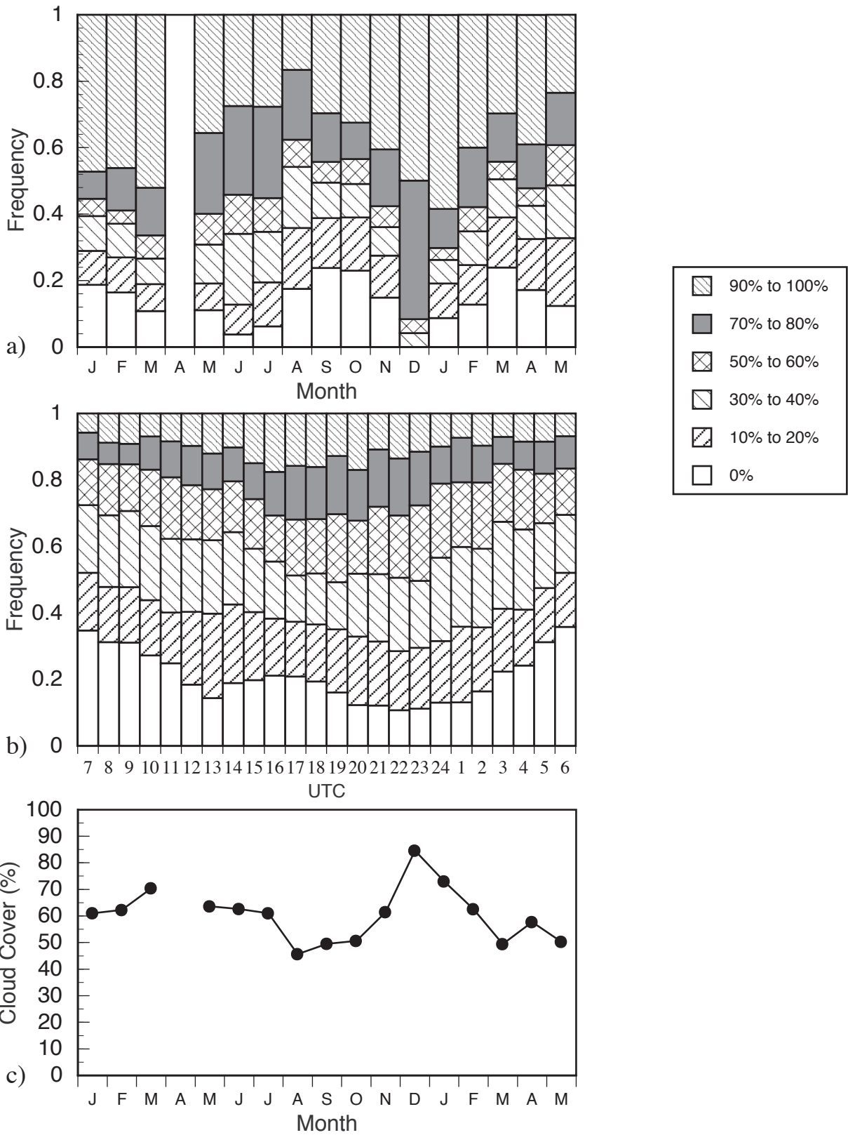
Figure C18. Summary of cloud cover for Whiteman AFB, Missouri from January 93 to May 94: (a) relative frequency of cloud cover, (b) diurnal cycle of cloud cover relative frequency centered at local noon, and (c) monthly mean cloud cover.
