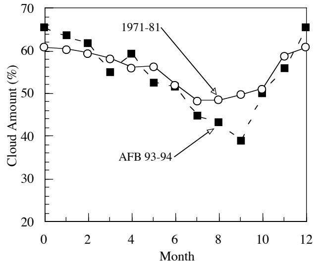
Fig. 12. Comparison of U.S. climatological average and contrail-data monthly mean cloud cover.
