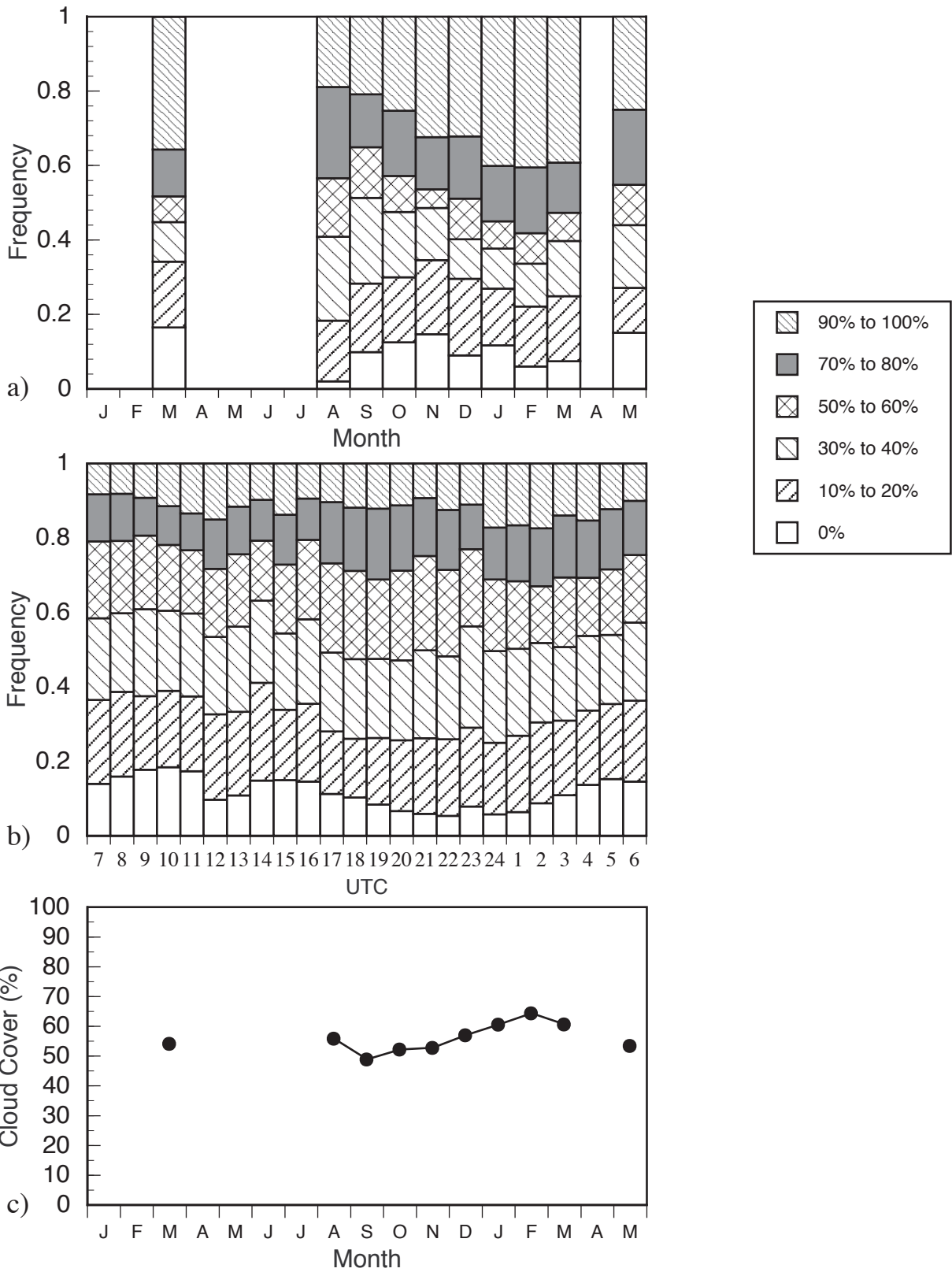
Figure C5. Summary of cloud cover for Eglin AFB, Florida from January 93 to May 94: (a) relative frequency of cloud cover, (b) diurnal cycle of cloud cover relative frequency centered at local noon, and (c) monthly mean cloud cover.
