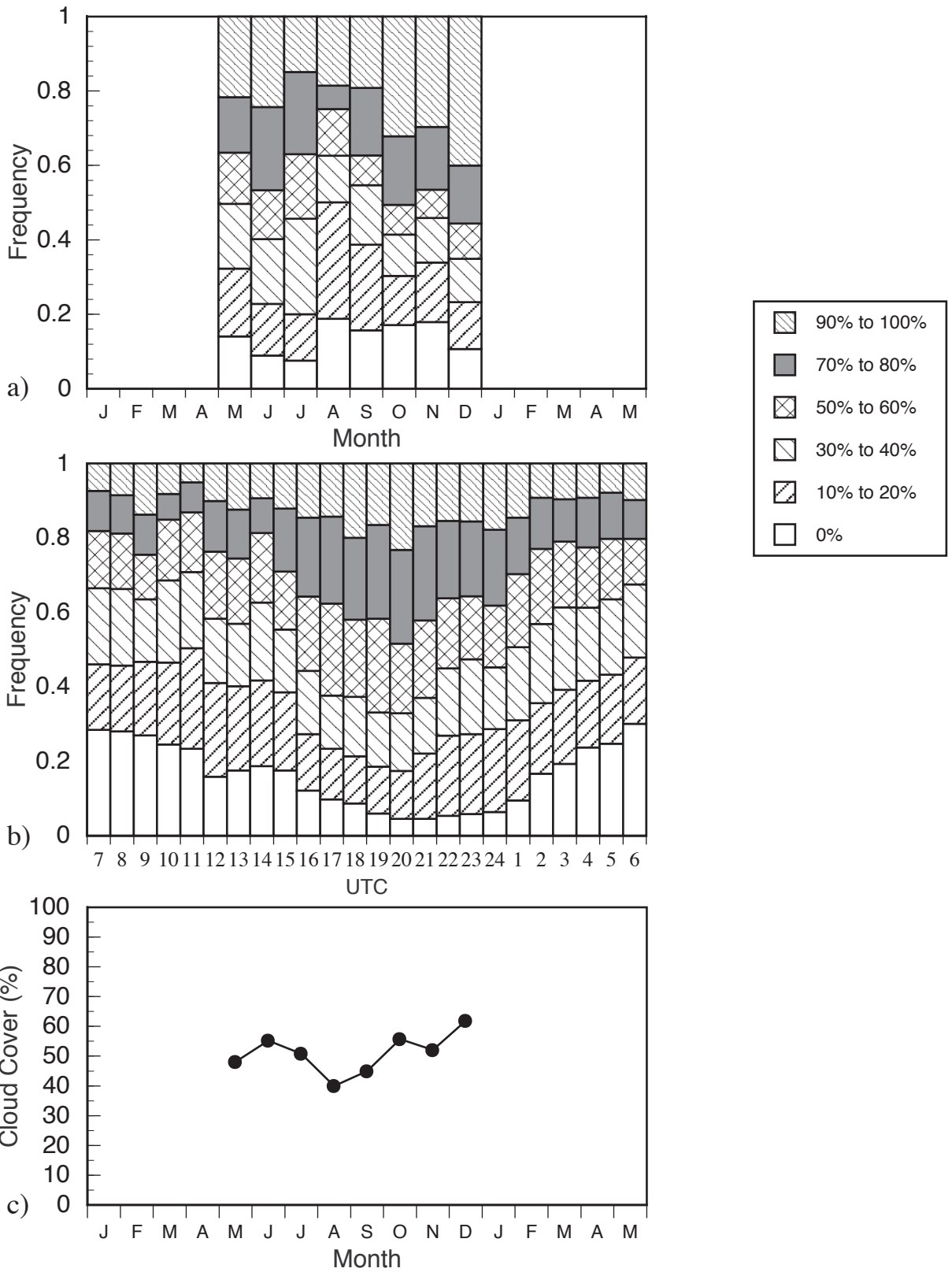
Figure C3. Summary of cloud cover for Cairns AAF, Alabama from January 93 to May 94: (a) relative frequency of cloud cover, (b) diurnal cycle of cloud cover relative frequency centered at local noon, and (c) monthly mean cloud cover.
