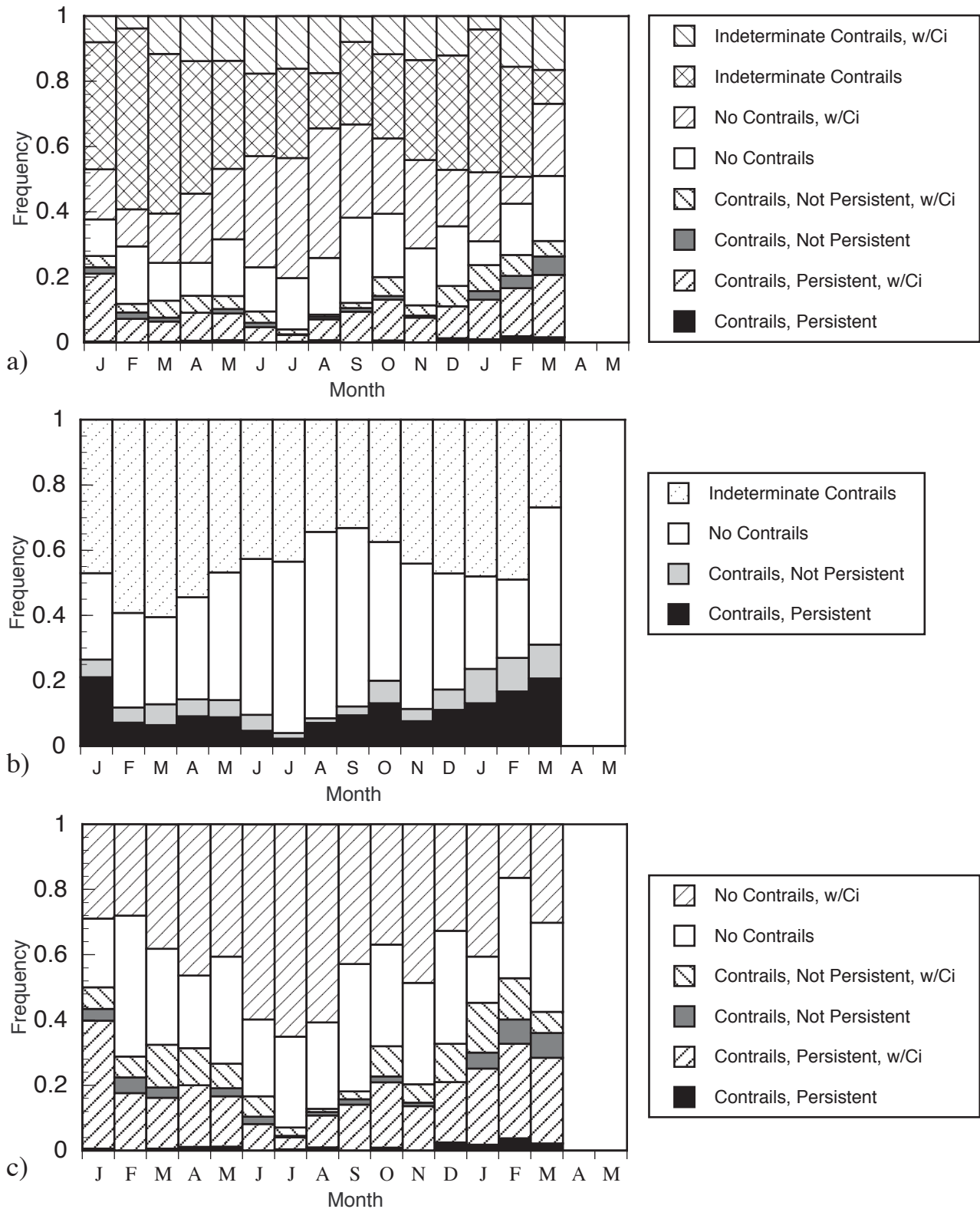
Figure A16. Summary of monthly observations for Offut AFB, Nebraska from January 93 to May 94: (a) relative frequency of contrails and cirrus, (b) relative frequency and persistence of contrails, and (c) relative frequency of contrails and cirrus with indeterminate data removed.
