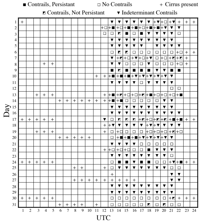
Figure 2. Coded summary of Langley AFB December 1993 contrail and cirrus observations.
