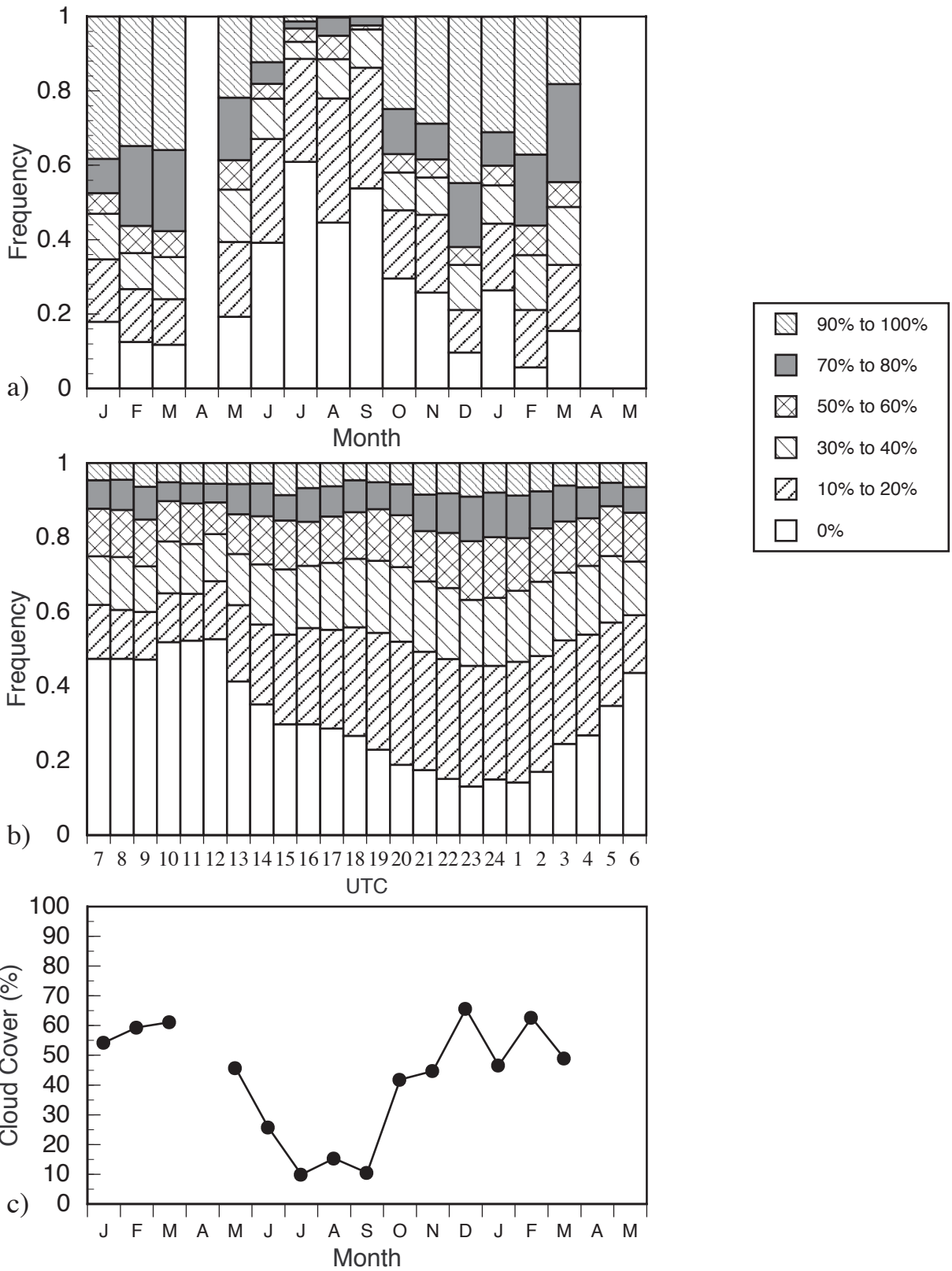
Figure C2. Summary of cloud cover for Beale AFB, California from January 93 to May 94: (a) relative frequency of cloud cover, (b) diurnal cycle of cloud cover relative frequency centered at local noon, and (c) monthly mean cloud cover.
