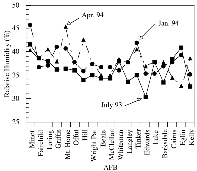
Figure 22. Comparison of mean relative humidities at 10.5 kilometer altitude for July 1993, January 1994, and April 1994. Sites ordered North to South according to latitude.
