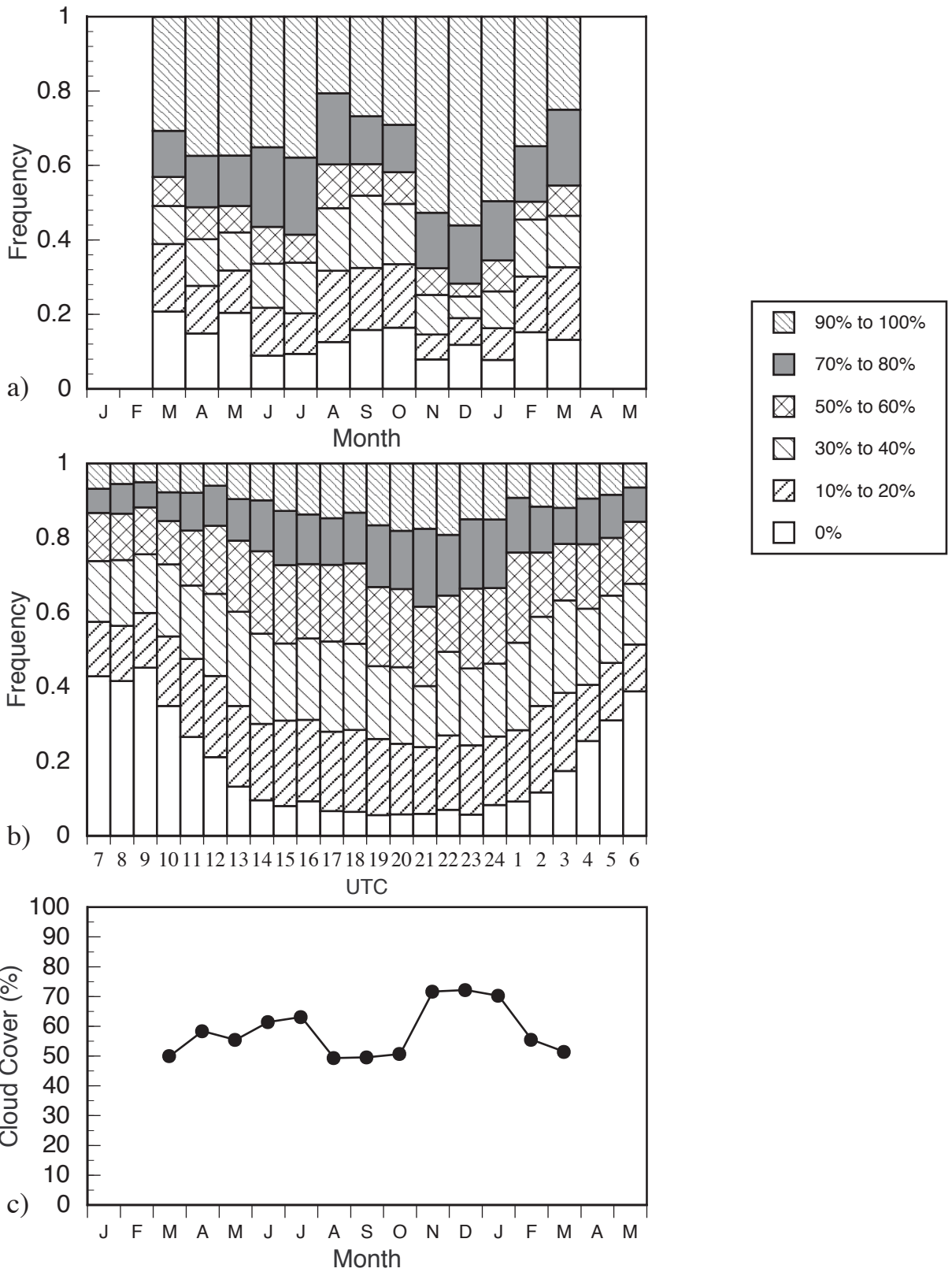
Figure C14. Summary of cloud cover for Minot AFB, North Dakota from January 93 to May 94: (a) relative frequency of cloud cover, (b) diurnal cycle of cloud cover relative frequency centered at local noon, and (c) monthly mean cloud cover.
