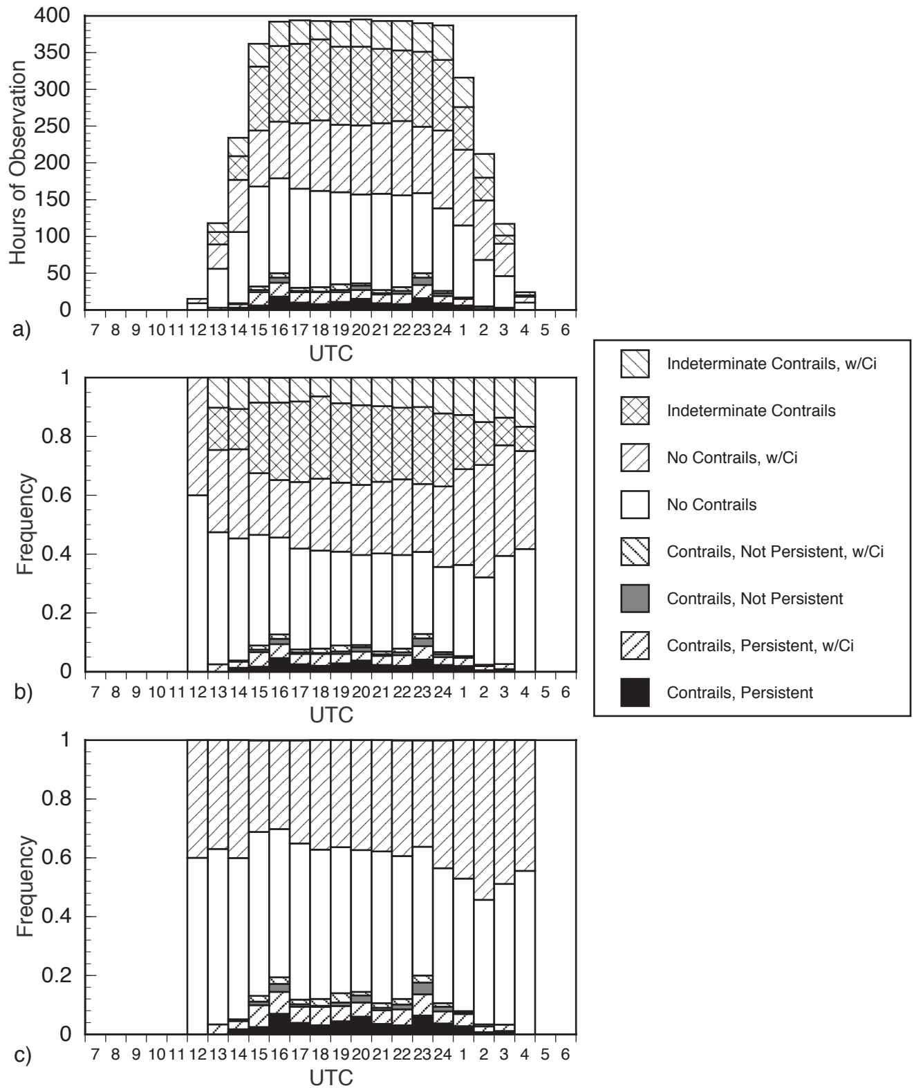
Figure B15. Summary of hourly contrail and cirrus observations from Mountain Home AFB, Idaho, centered at local noon: (a) number of observations, (b) relative frequency of occurrence, and (c) relative frequency of occurrence with indeterminate data removed.
