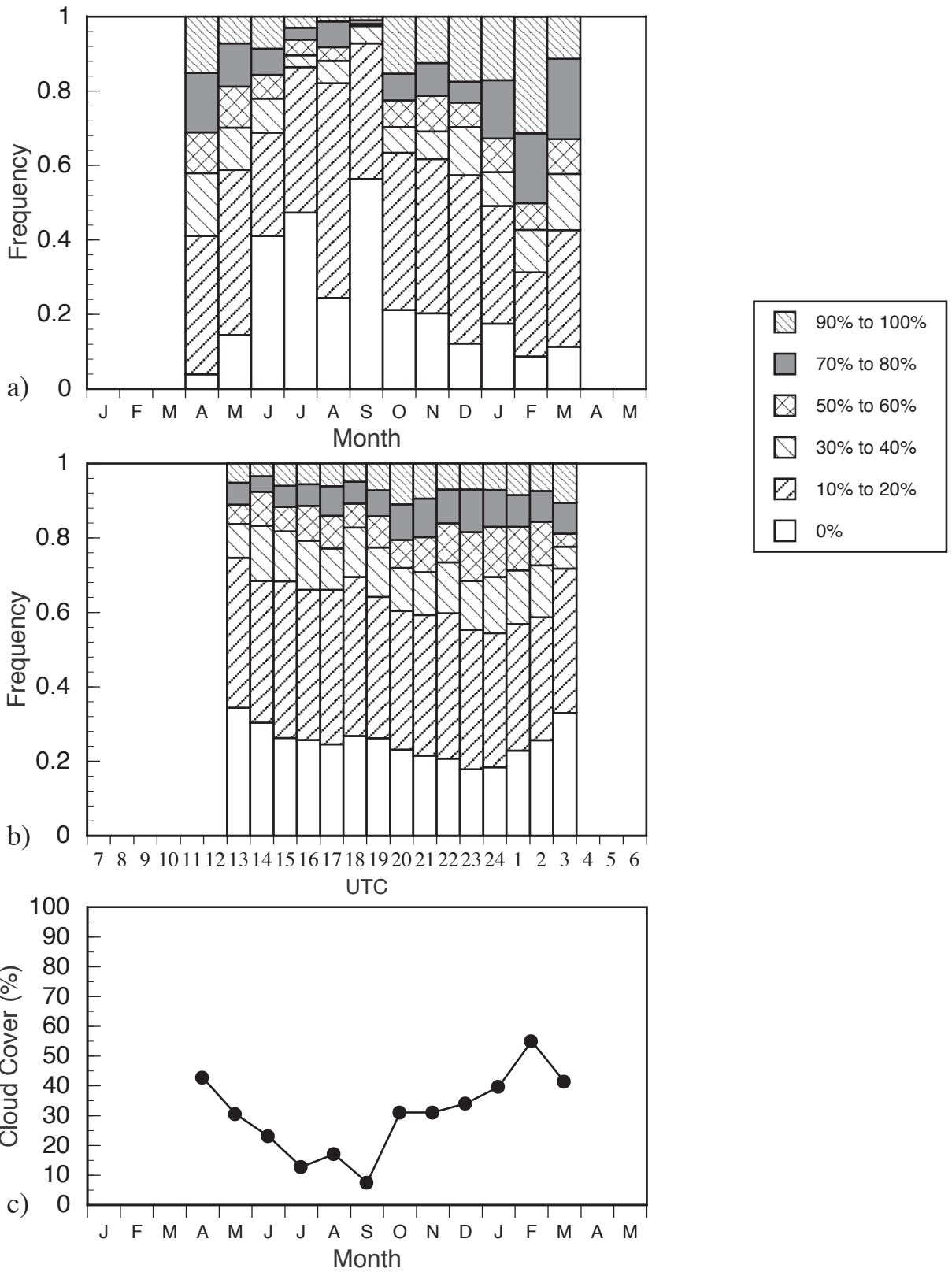
Figure C4. Summary of cloud cover for Edwards AFB, California from January 93 to May 94: (a) relative frequency of cloud cover, (b) diurnal cycle of cloud cover relative frequency centered at local noon, and (c) monthly mean cloud cover.
