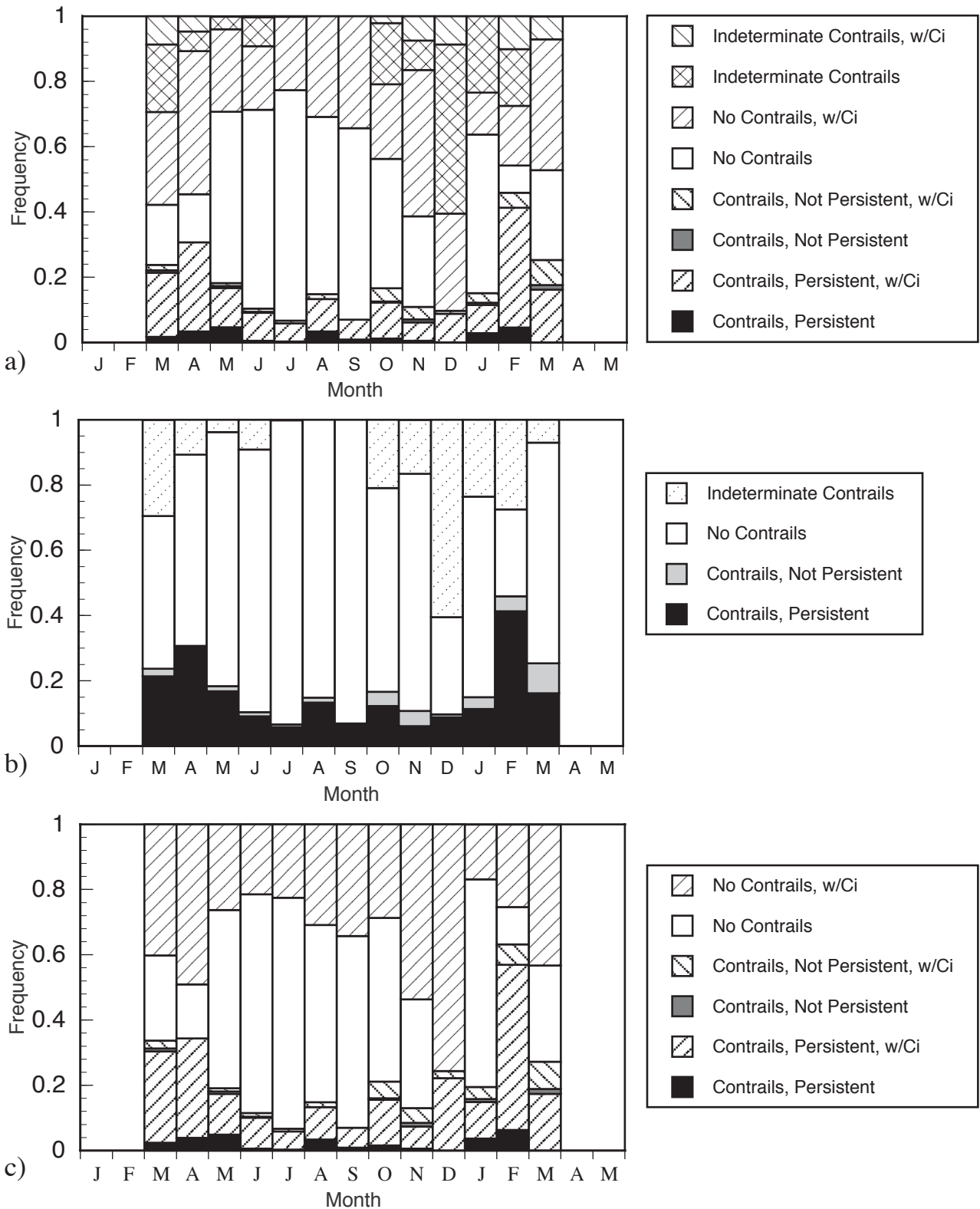
Figure A13. Summary of monthly observations for McClellan AFB, California from January 93 to May 94: (a) relative frequency of contrails and cirrus, (b) relative frequency and persistence of contrails, and (c) relative frequency of contrails and cirrus with indeterminate data removed.
