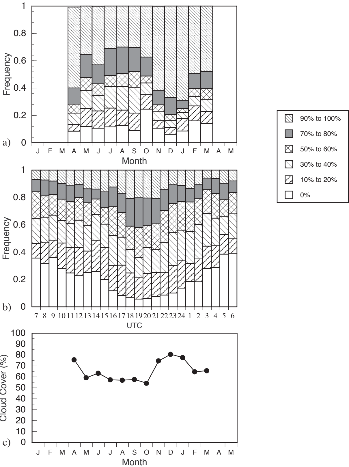
Figure C19. Summary of cloud cover for Wright Patterson AFB, Ohio from January 93 to May 94: (a) relative frequency of cloud cover, (b) diurnal cycle of cloud cover relative frequency centered at local noon, and (c) monthly mean cloud cover.
