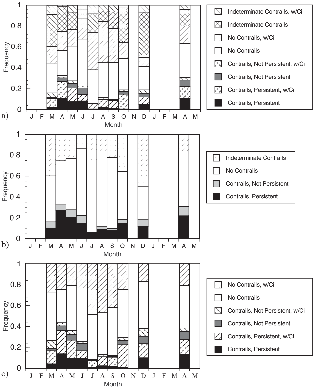
Figure A10. Summary of monthly observations for Langley AFB, Virginia from January 93 to May 94: (a) relative frequency of contrails and cirrus, (b) relative frequency and persistence of contrails, and (c) relative frequency of contrails and cirrus with indeterminate data removed.
