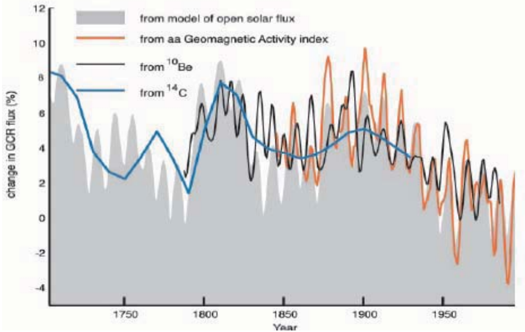
Figure 2- Fluctuations in Cosmic Ray Flux
