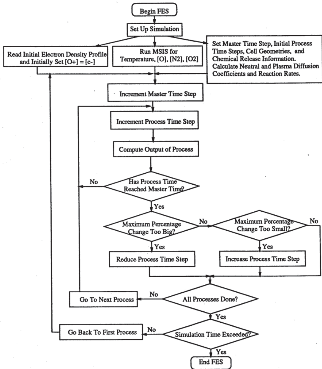
Figure 4: FES functional flow chart.
