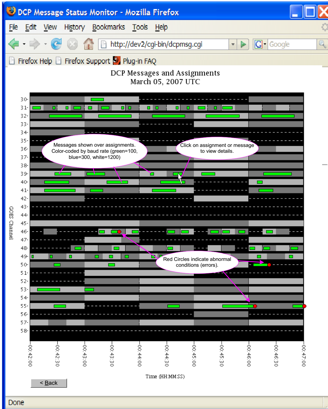
Figure 11: DCP Monitor - Graphic Time-Slot Viewer.
