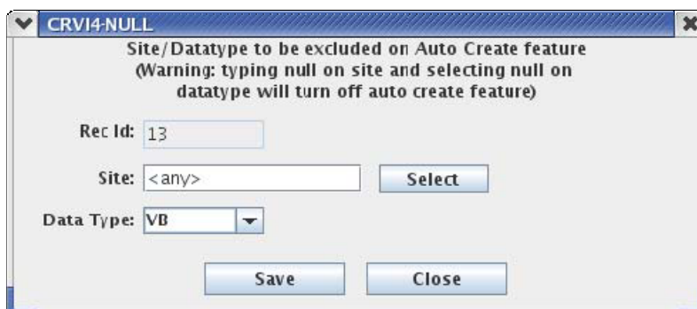
Figure 5: Create Rules to Control how DECODES Auto-Creation is Done.
