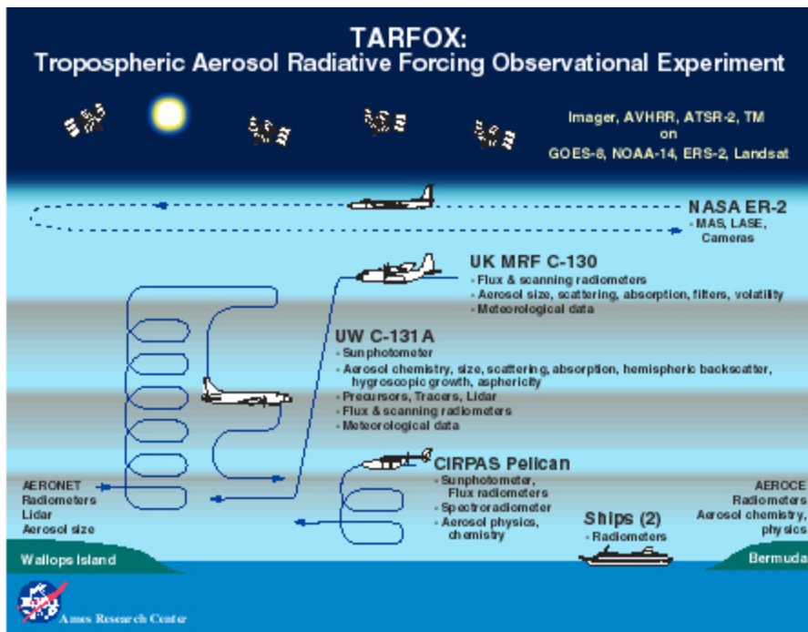
Plate 2. Schematic overview of TARFOX platforms, instruments, and experimental approach.
