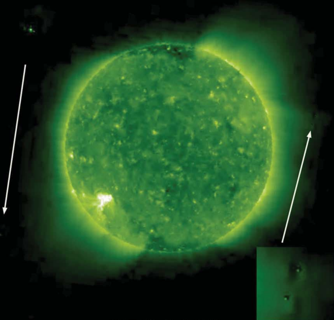
STEREO Behind EUVI 195
