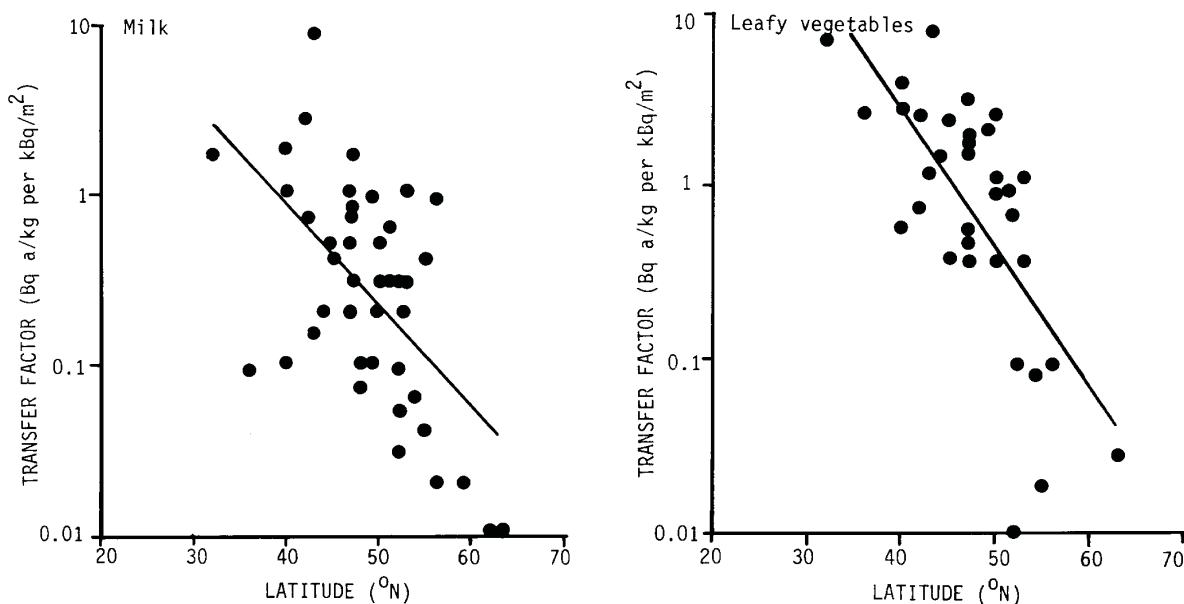
Figure VIII. Integrated concentrations of ^{131}\text{I} in milk and leafy vegetables per unit ^{131}\text{I} deposition density.
