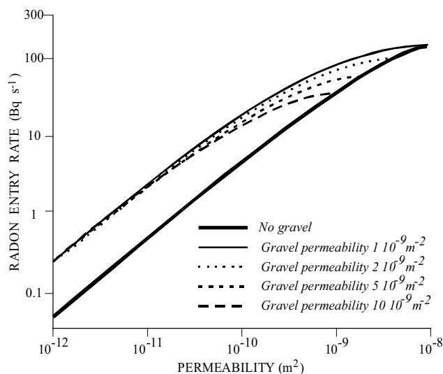
Figure XI. Advective radon entry rates into a typical basement [R15]. Assumes slab-to-wall gap of 3 mm, deep soil radon concentration of 37 \text{ kBq m}^{-3} , gravel layer beneath basement slab of thickness of 15 cm and basement pressure of -5 \text{ Pa} with respect to the atmosphere.
