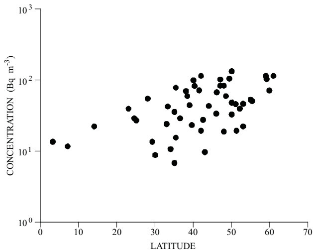
Figure XIII. Average concentrations of radon indoors in various countries in which measurements have been made in relation to latitude.
