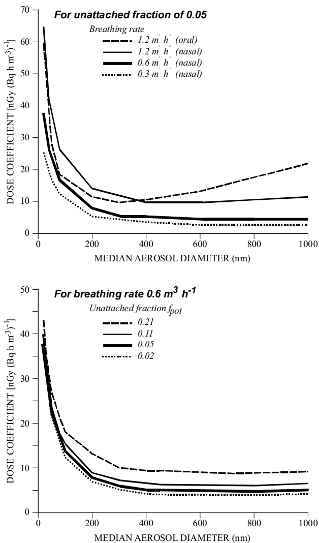
Figure XIV. Absorbed dose in bronchial epithelial cells per unit exposure (EEC) to radon.
