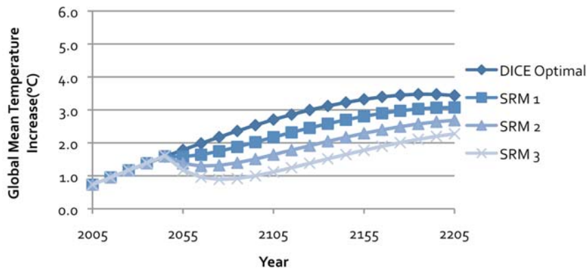
Figure 6: Optimal Controls temperature changes (°C) with the year 2055 deployment of SRM.
