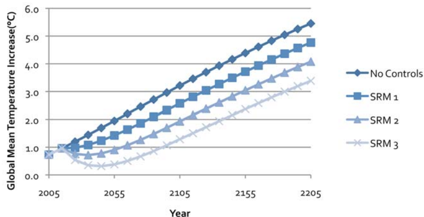
Figure 1: No Controls temperature changes ( ^\circ\text{C} ) with the deployment of SRM.
