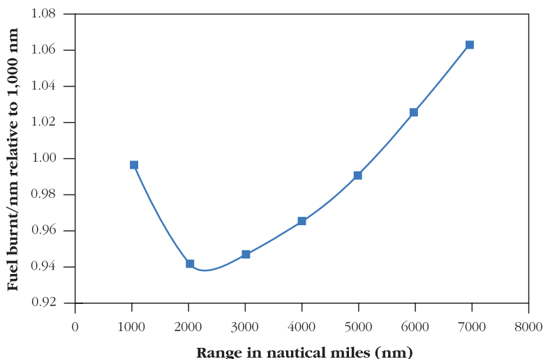
Figure 4-II Average fuel use per passenger-kilometre for flights of varying length
