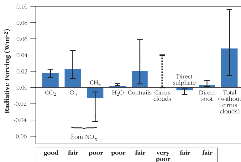
Figure 3-I Radiative forcing from aviation effects in 1992
