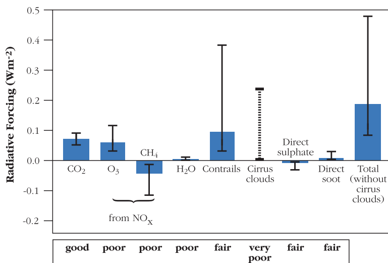
Figure 3-III Predicted radiative forcing from aviation effects in 2050
