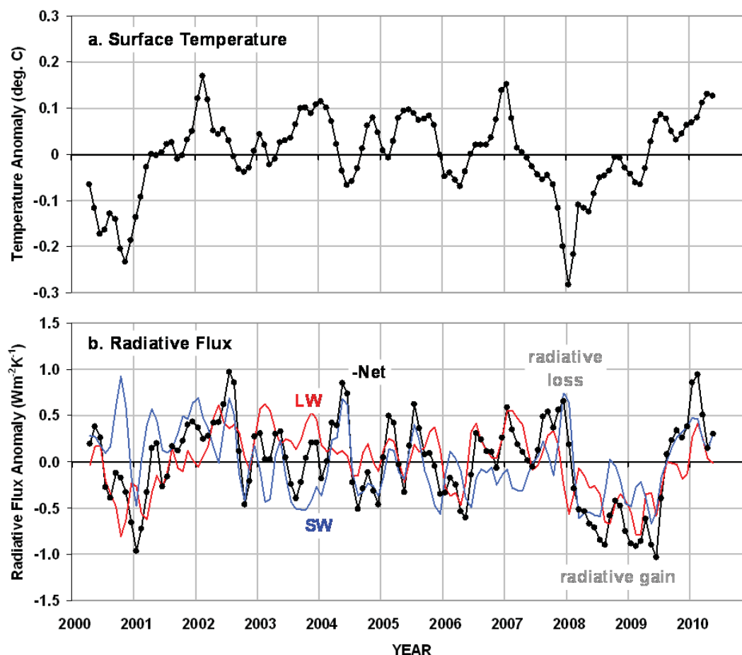
Figure 2. Times series of monthly global average anomalies in (a) surface temperatures from HadCRUT3, and (b) radiative fluxes from Terra CERES SSF Edition 2.5, for the period March 2000 through June 2010. All time series have a 1-2-1 smoother applied to reduce sampling noise.
