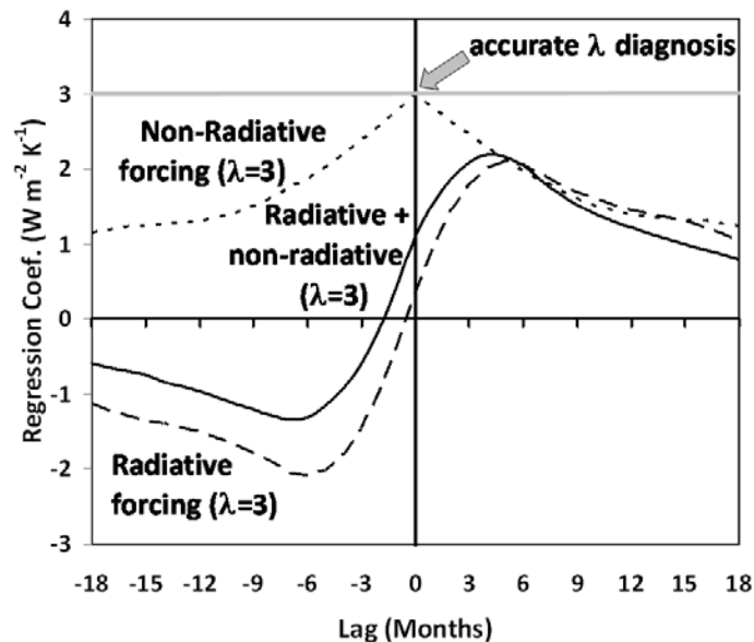
Figure 4. Lag regression coefficients between temperature and radiative flux from the simple forcing-feedback model run for three forcing cases: pure non-radiative forcing (dotted line); pure radiative forcing (dashed line); and a 70% radiative/30% non-radiative forcing mixture. A feedback parameter of 3 \text{ W m}^{-2} \text{ K}^{-1} and ocean mixing depth of 25 m were specified for all three simulations, which each ran for 500 years of simulated time.
