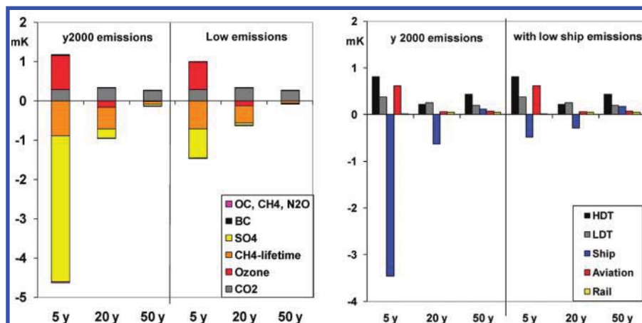
FIGURE 2. Comparison of temperature change for various years after the emissions due to ship emissions with standard y2000 emissions and with reduced \text{SO}_2 (-80%) and \text{NO}_x (-20%) emissions. Temperature change per compound for shipping (left); temperature change of freight modes (right).
