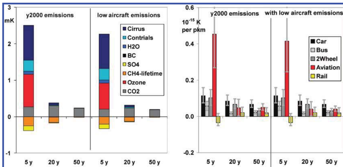
FIGURE 4. Comparison of temperature change for various years after the emissions due to aviation with standard emissions for the year 2000 and with reduced CO 2 and NO x emissions (-20%). Temperature change per compound (left); specific climate impact of passenger modes per passenger-kilometer (right).
