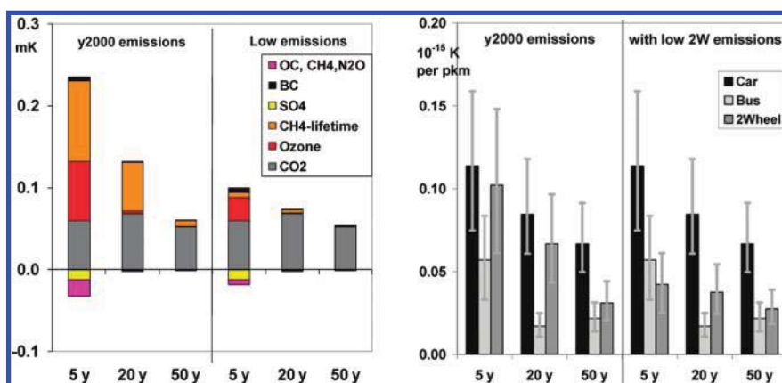
FIGURE 3. Comparison of temperature change for various years after the emissions due to motorized two- and three-wheelers with standard emissions for the year 2000 and with reduced emissions (CO, VOC, OC: -80%). Temperature change per compound (left); specific climate impact of road passenger modes per passenger-km (right).
